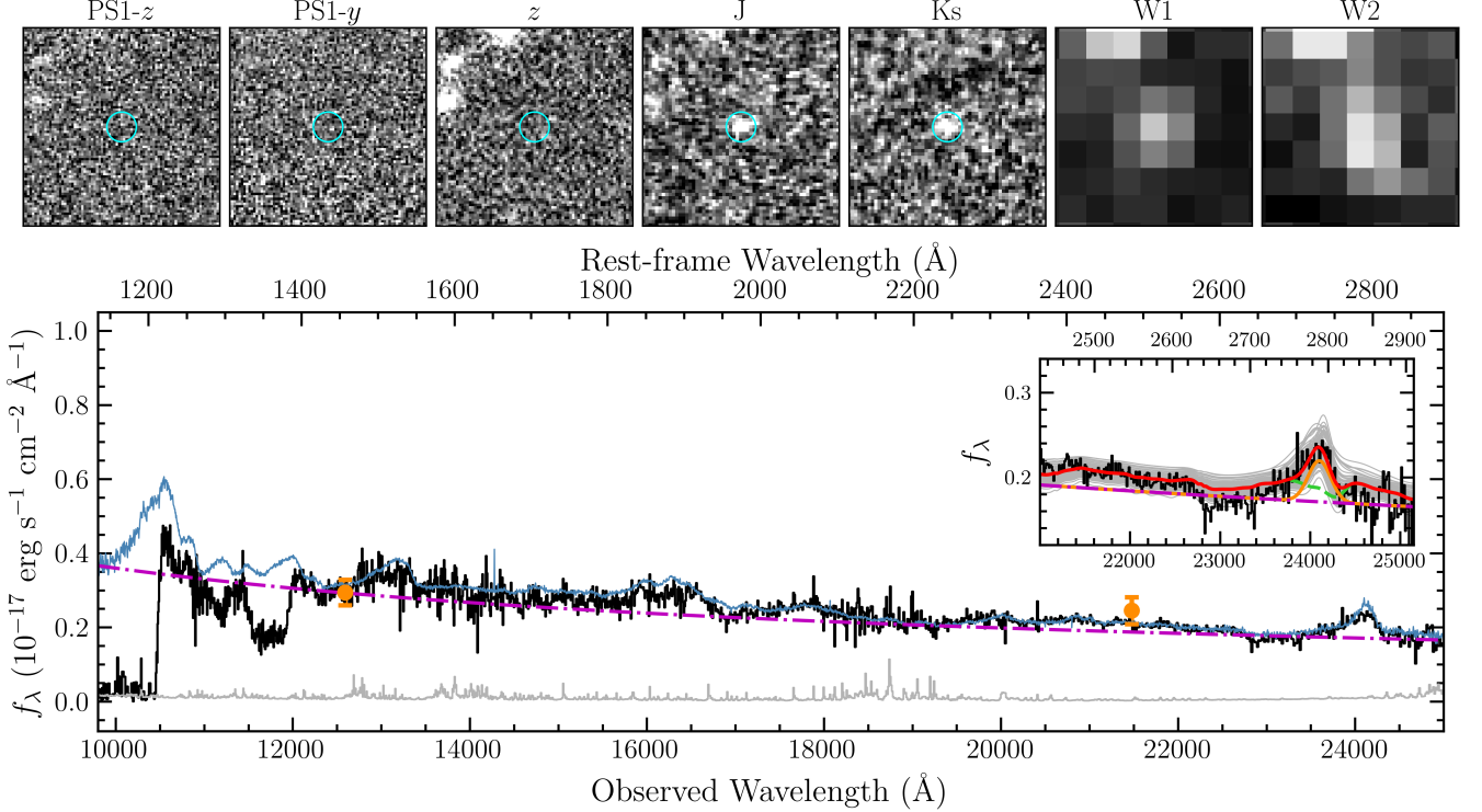
Figure 1. Upper panel: image cutouts ( 20'' \times 20'' , north is up and east is to the left) for J0313–1806 in PS1 z , PS1 y , DELS z , VISTA J , VISTA Ks , WISE W1 and WISE W2 bands. The photometry is given in Table 1. Lower panel: the final stacked spectrum of J0313–1806. In the figure, we re-binned the spectrum by two spectral pixels ( \sim 173 \text{ km s}^{-1} ) for illustration purposes. The black and gray lines represent the Galactic extinction-corrected spectrum and the error vector, respectively. The blue line denotes the quasar composite spectrum constructed with SDSS z \sim 2 quasars having similar C IV blueshifts and line strengths. The purple dashed line denotes the power-law continuum. The orange points are flux densities determined from photometry in the J and Ks -bands. The inset panel shows the Mg II line fitting with the purple dot-dashed line denoting the power-law continuum, the green dashed line denoting the pseudo-continuum model (the sum of power law continuum, Fe II emission, and Balmer continuum), the orange line representing the Gaussian fitting of the Mg II line and the red line representing the total fit of pseudo-continuum and Mg II line. The thin grey lines in the insert panel represent the spectral fitting of 100 mock spectra as described in §3.
