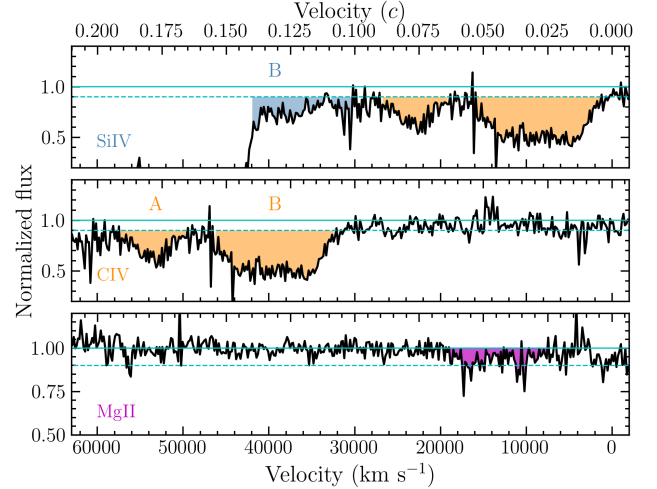
Figure 4. The normalized spectrum of J0313–1806. The solid and dashed lines represent 100% and 90% of the normalized spectrum, respectively. The top panel shows the outflow velocity of the Si IV line, the middle panel denotes the outflow velocity of the C IV line, and the bottom panel represents the outflow velocity of the Mg II line. We interpret the two most obvious troughs (orange regions) as extremely high velocity C IV outflow systems with trough A having v = (0.171 - 0.186)c and trough B having v = (0.109 - 0.155)c . There is a potential weak Mg II absorption trough (the highlighted purple region in the bottom panel), but it does not satisfy the BI definition.
