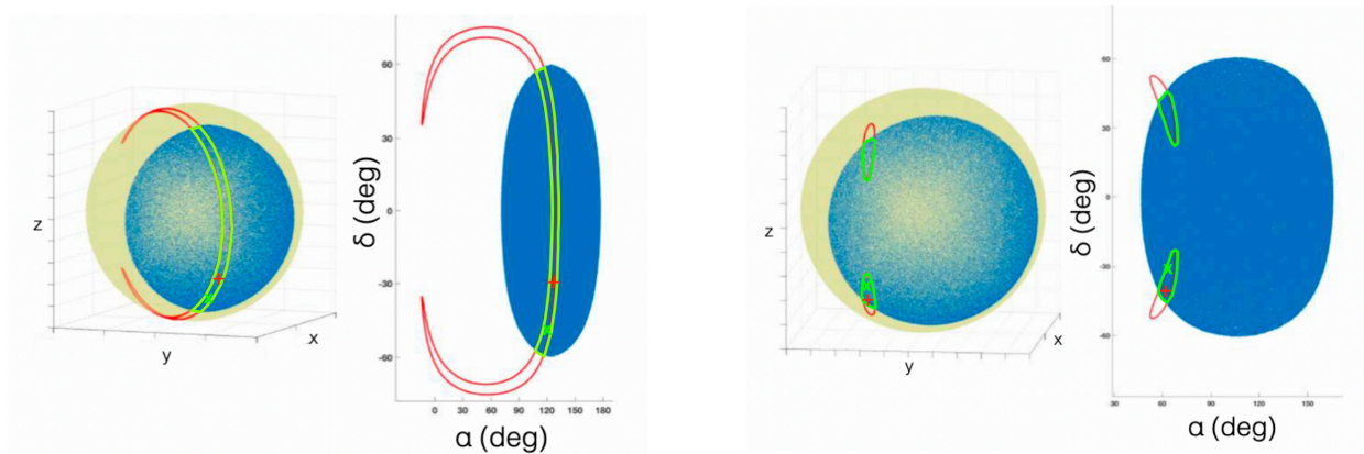
Figure 8. Example of GRB localization obtained by simulating a GRB with latitude \lambda 30 deg (left panel) and latitude \lambda 70 deg (right panel). The GRB position and best-fit position are represented with the green X-symbol and the red +symbol, respectively. The red contour line shows the 1\sigma confidence level region associated with the best fit position. The blue-filled region represents the overlapping FoVs of the 3 satellites observing simultaneously the GRB. The light-green contour line shows the 1\sigma confidence level region corrected to take into account the FoVs of the detectors.
