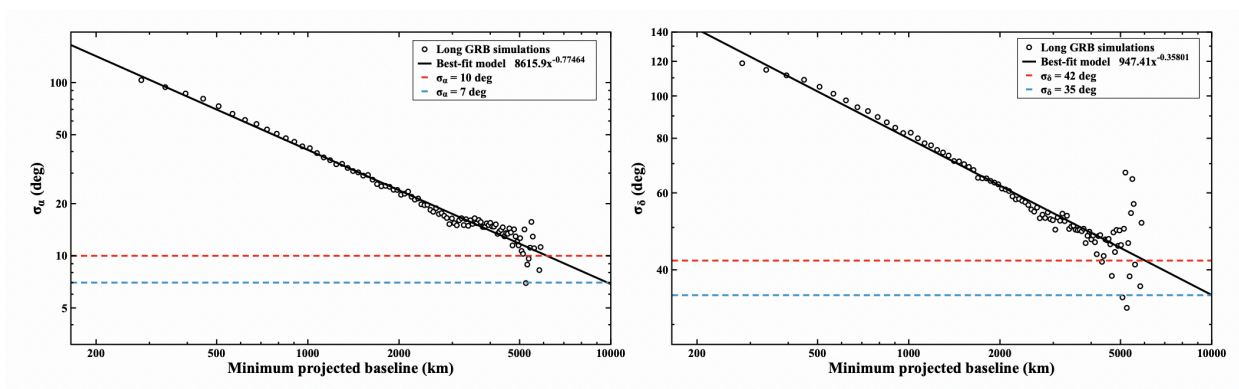
Figure 12. Average correlation between the uncertainties in the Right Ascension \sigma_\alpha (left panel) and Declination \sigma_\delta (right panel) coordinates as a function of the minimum projected baseline obtained by binning the results from the simulated long GRB as detected by the HTP/HSP mini-constellation. The black-solid lines represent the best-fitting model to the data, whilst dashed red and cyan lines mark the achievable values of \sigma_\alpha and \sigma_\delta for minimum projected baselines of 6000 km and 10000 km, respectively.
