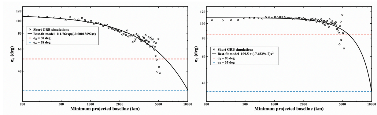
Figure 13. Average correlation between the uncertainties in the Right Ascension \sigma_\alpha (left panel) and Declination \sigma_\delta (right panel) coordinates as a function of the minimum projected baseline obtained by binning the results from the simulated short GRB as detected by the HTP/HSP mini-constellation. The black-solid lines represent the best-fitting model to the data, whilst dashed red and cyan lines mark the achievable values of \sigma_\alpha and \sigma_\delta for minimum projected baselines of 6000 km and 10000 km, respectively.
