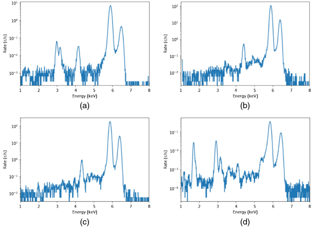
Fig. 10 Spectra of elements of FCS FM2 acquired with Amptek XR-100SDD SDD. (a) Spectrum of CalA2: the closely packed peaks of the AgL_{\alpha} and L_{\beta} lines at 2.98 and 3.15 keV are visible, as are the 5.9-keV Mn K_{\alpha} line and its escape at 4.2 keV and the K_{\beta} line at 6.5 keV; (b) spectrum of CalB2; (c) spectrum of CalC2: the 5.9-keV Mn K_{\alpha} line and its escape at 4.2 keV as well as the Mn K_{\beta} line at 6.5 keV are visible in both spectra; and (d) spectrum of CalD: the lines at \sim 3 keV due to argon in the air are well distinguished, similar to the 1.7-keV Si fluorescence.
