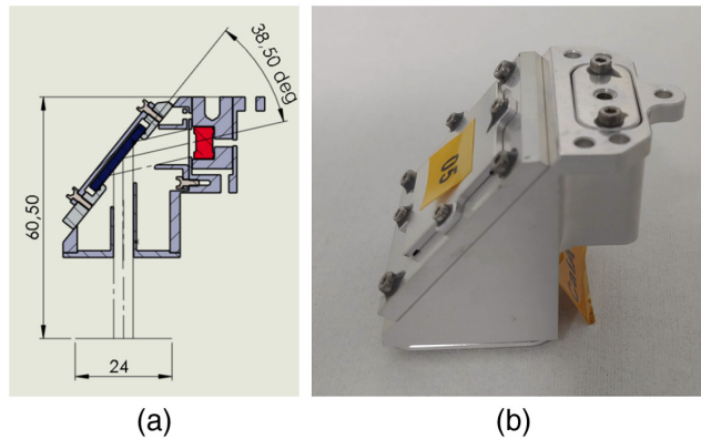
Fig. 2 The polarized on-board calibration source Cal A enables production of polarized x-ray photons of known energy. (a) Cross-sectional view of CalA: the 55 Fe radioactive source is shown in red; a thin silver foil is placed in front to extract 3.0 keV fluorescence. The graphite mosaic crystal for Bragg diffraction is shown in dark blue. Numbers are in mm. (b) Picture of CalA.
