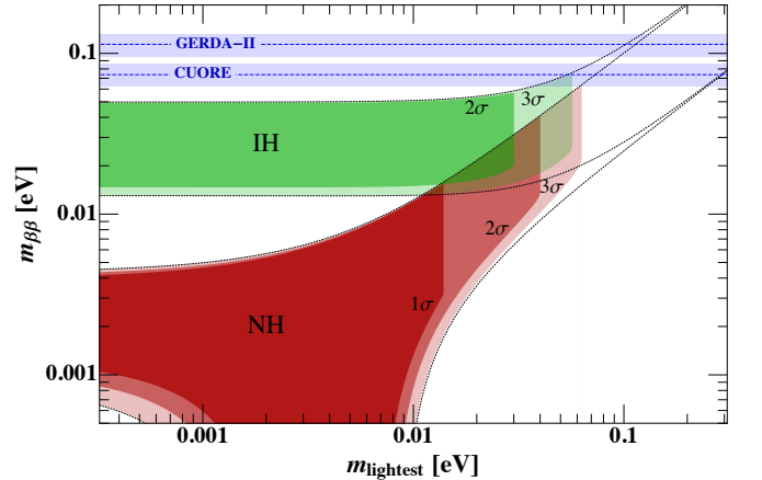
FIG. 2. Constraints from cosmological surveys are added to those from oscillations in the representation m_{\beta\beta} as a function of the lightest neutrino mass. The dotted contours represent the 3\sigma regions allowed considering oscillations only. The shaded areas show the effect of the inclusion of cosmological constraints at different C.L.. The horizontal bands correspond to the expected sensitivity for future experiments, according to Ref. [3].
