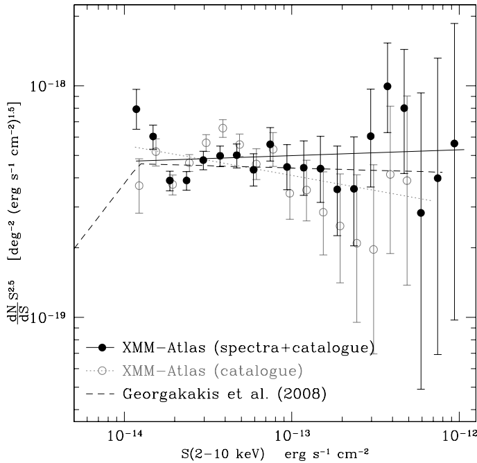
Fig. 8. XMM-ATLAS log N –log S in the 2–10 keV band. Filled circles: fluxes from the spectral fits are used whenever possible; catalogue fluxes are used otherwise. Open circles: only fluxes from the catalogue are used; a small horizontal shift has been introduced in the plot to better distinguish the error bars. The solid line shows the best fit to the filled data points. The dashed line is the best-fit model from Georgakakis et al. (2008). The error bars show the 1\sigma uncertainty.
