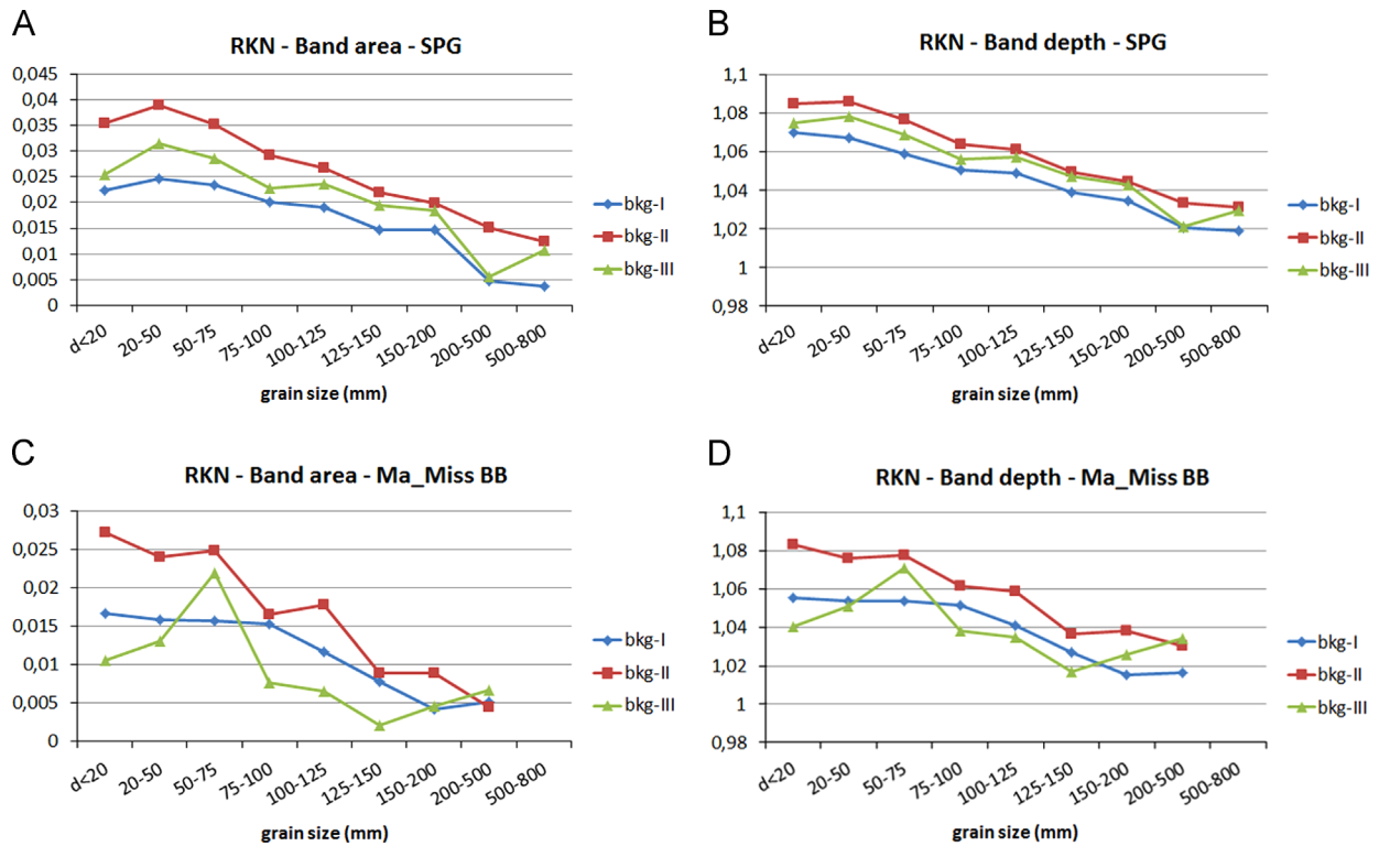
Fig. 6. Sample RKN. A and C: band area at 1 \mu\text{m} computed from SPG and Ma_Miss data, respectively, using three different polynomials as continuum background (straight line (I), parabolic (II) and cubic (III)). B and D: band depth at 1 \mu\text{m} computed from SPG and Ma_Miss data, respectively, using three different polynomials as continuum background.
