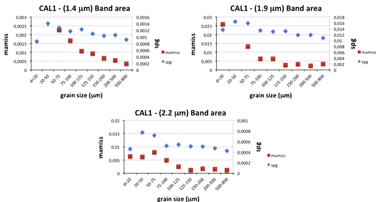
Fig. 13. Sample CAL1. Band area of absorptions at 1.4 \mu\text{m} (A), 1.9 \mu\text{m} (B), 2.2 \mu\text{m} (C).
