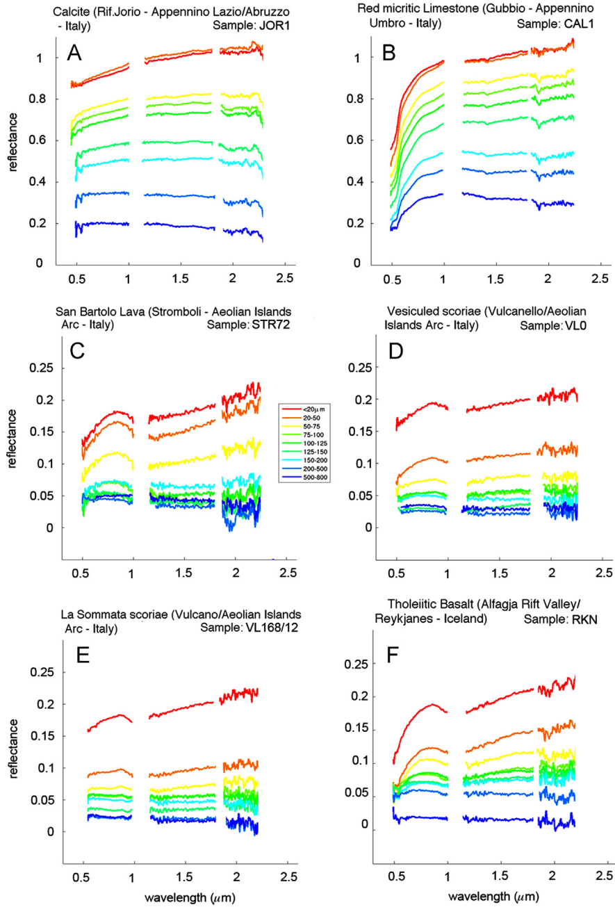
Fig. 3. Reflectance spectra acquired with Ma_Miss breadboard setup. The spectra acquired with Ma_Miss BB setup show two gaps in the data at around 1 \mu\text{m} and 1.8 \mu\text{m} , because data are too noisy at the juncture between the Fieldspec's detectors. See the text for more details.
