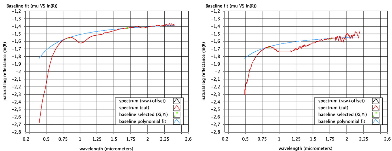
Fig. 4. Example of continuum background subtraction, for the sample RKN ( d < 20 \mu\text{m} ; left: SPG. Right: Ma_Miss BB). Here the feature to analyze is the 1\text{-}\mu\text{m} band: the extremes (green squares) have been set at 0.85 and 1.7 \mu\text{m} . The continuum (blue curve) is a straight line in the \ln R vs. wavenumber space, while it is a logarithm in the \ln R vs. wavelength space. (For interpretation of the references to color in this figure legend, the reader is referred to the web version of this article.)
