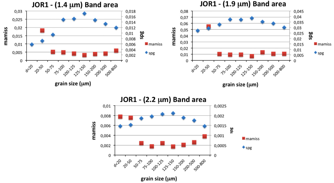
Fig. 16. Sample JOR1. Band area of absorptions at 1.4 \mu\text{m} (A), 1.9 \mu\text{m} (B), and 2.2 \mu\text{m} (C).
