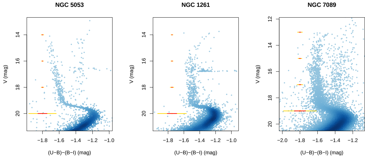
Figure 11. Examples of V , C_{UBI} CMDs for three well-known GCs that were not included in the sample presented by Monelli et al. (2013), sorted by RGB width and complexity. Left panel: NGC 5053, one of the most metal-poor GCs displaying one of the thinnest RGBs in our sample, although still a few times wider than the typical photometric errors. Center panel: the beautiful substructure of the RGB of NGC 1261, a low-reddening GC. Right panel: the complex structure of another anomalous GC, NGC 7089 (M 2), containing a small fraction of s-rich and C+N+O enhanced stars, which are however not clearly visible in C_{UBI} . In all panels, median errorbars are displayed in gold ( 3\sigma ) and red ( 1\sigma ) at different magnitude levels.
