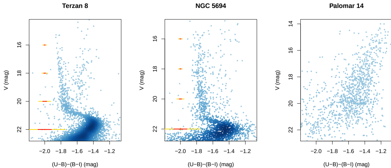
Figure 12. The V , C_{UBI} CMDs of candidate single-population or mostly single-population GCs in our sample. As in Figure 11, median errorbars at different magnitude levels are shown in gold ( 3\sigma ) and red ( 1\sigma ). Unfortunately, the current U -band photometry of Palomar 14 is not deep enough to study MPs.
