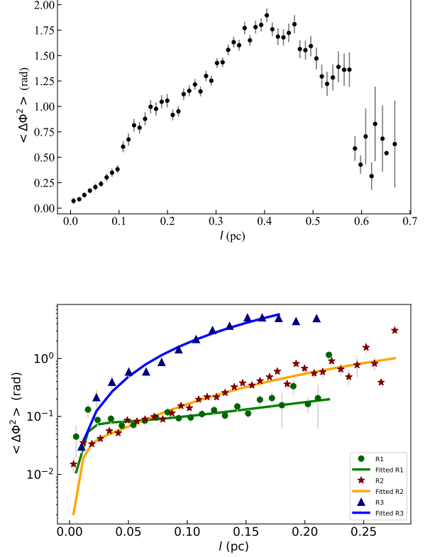
Fig. 7: ADF versus distance, l . Top panel: ADF for the whole filament. Bottom panel: Same but for the three filament regions. The best fits to the data points using Eq. (9) for R1, R2, and R3 are shown with the green, orange, and blue curves, respectively. Measurement uncertainties are displayed as error bars, which are not visible for small values of l due to the higher statistics.
