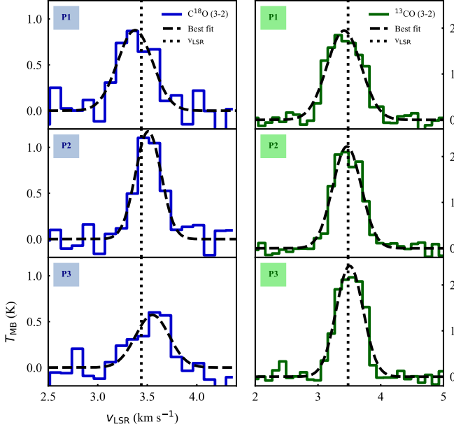
Fig. 3: C^{18}O (3-2) and ^{13}CO (3-2) spectra at three selected locations within the filament (locations are shown with blue crosses in Fig. 2). C^{18}O (3-2) spectra are in the left column, and ^{13}CO (3-2) spectra are in the right column. Blue and green lines show the observed spectra for the C^{18}O and ^{13}CO , respectively, whereas dashed black curves show the best-fit Gaussian for each. As displayed by the vertical dotted lines, C^{18}O (3-2) and ^{13}CO (3-2) have average V_{lsr} of 3.4 and 3.5 km\ s^{-1} , respectively.
