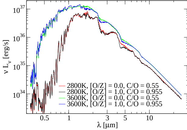
Figure B1. Spectra based on COMARCS models with T_{\text{eff}} = 2800 K or 3600 K, \log(g [\text{cm/s}^2]) = 0.0 , one solar mass and solar metallicity. The effect of changing [O/Z] from 0 to +1 at a constant (O-C) of 8.455 is shown.
