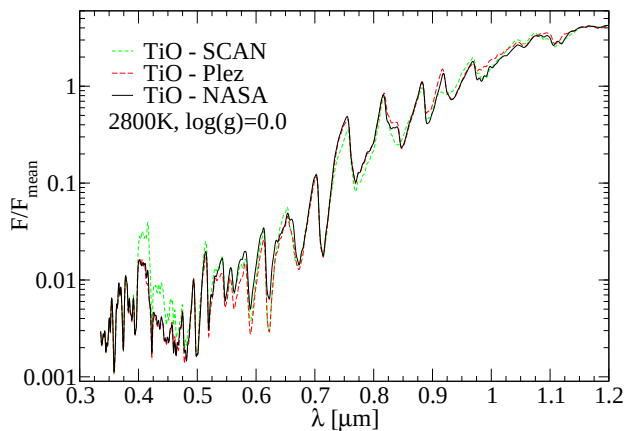
Figure 2. Spectra calculated with different TiO data based on a COMARCS model with T_{\text{eff}} = 2800 K, \log(g [\text{cm/s}^2]) = 0.0 , one solar mass and solar metallicity. The NASA-AMES (black, used in this work as standard), Plez (red) and SCAN (green) line lists are compared. The intensities \nu L_\nu are normalized to their mean value.
