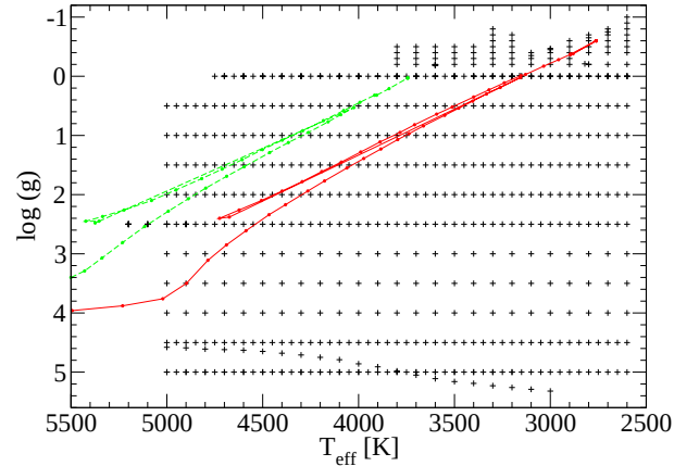
Figure 4. Values of effective temperature and \log(g [\text{cm/s}^2]) covered by the current COMARCS grid in the case of solar abundances (crosses). Models of different mass are not distinguished. In addition, evolutionary tracks for stars with one solar mass and Z/Z_{\odot} = 1.0 (full line, red) as well as Z/Z_{\odot} = 0.1 (dashed line, green) are displayed.
