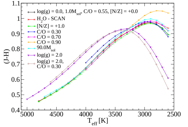
Figure 12. (J-H) as a function of the effective temperature for COMARCS models with solar metallicity. Parameters, symbols and lines are like in Fig. 11.
