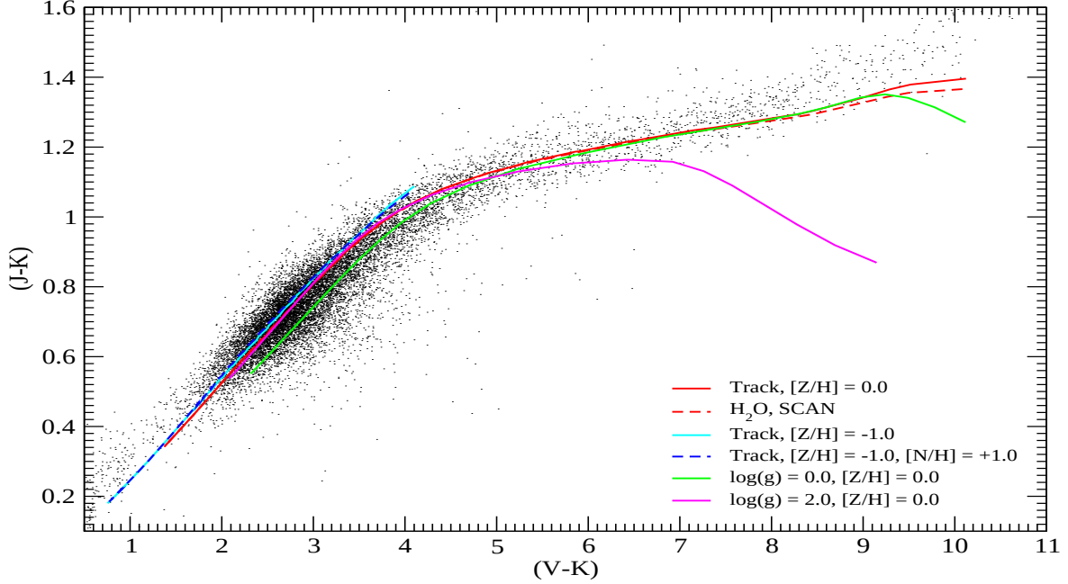
Figure 15. Two colour diagram ( J-K ) versus ( V-K ) for different sequences of COMARCS atmospheres. Models placed along evolutionary tracks for stars with one solar mass and Z/Z_{\odot} = 1.0 (full line, red) as well as Z/Z_{\odot} = 0.1 (full line, cyan) are displayed (see Fig. 4). For the solar metallicity track we show the effect of using the SCAN data for water (dashed line, red) and for the metal-poor one the result of increasing nitrogen by a factor of ten ( [N/Z] = +1 , dashed line, blue). In addition, two sequences of models having solar mass and abundances with \log(g \text{ [cm/s}^2\text{]}) = 0.0 (full line, green, T_{\text{eff}} 2600 to 4800 K) and \log(g \text{ [cm/s}^2\text{]}) = 2.0 (full line, magenta, T_{\text{eff}} 2600 to 5000 K) are included. The dots represent cool giants in Baade’s window (black) and Mira variables (orange) in the Galactic Bulge.
