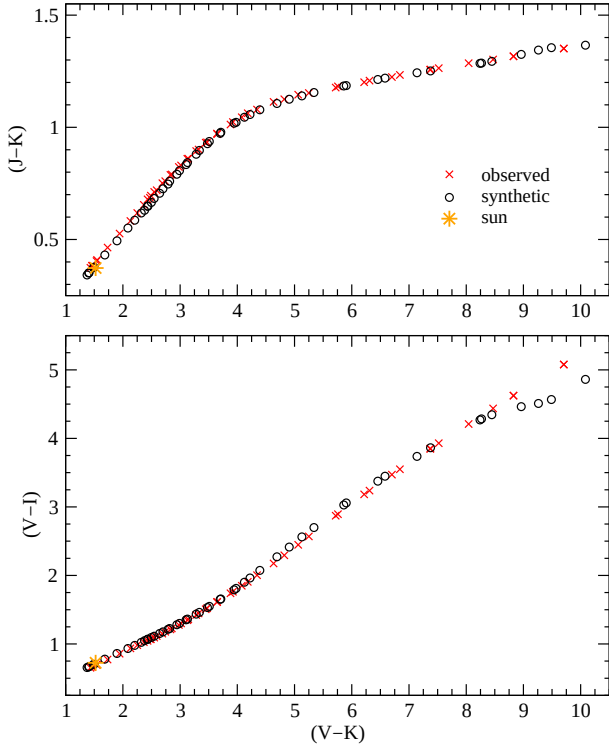
Figure 13. Two colour diagrams ( J-K ) and ( V-I ) versus ( V-K ) for stars placed along an evolutionary track with one solar mass and Z/Z_{\odot} = 1.0 (see Fig. 4). The results for a sequence of CO-MARCS models (black circles) are compared to the corresponding values taken from the fit routines by Worthey & Lee (2011), which are based on a large collection of observational material (red crosses). The colours of the Sun according to Bessell et al. (1998) are also shown (yellow stars).
