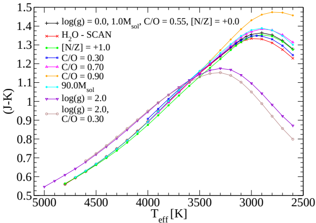
Figure 11. (J-K) as a function of the effective temperature for COMARCS models with solar metallicity. The standard parameters are \log(g \text{ [cm/s}^2\text{]}) = 0.0 , M/M_\odot = 1.0 , solar abundances ( C/O = 0.55 , [N/Z] = 0.0 ) and usage of the BT2 linelist for water below 4000 K (black). The result of changing C/O to 0.3 (blue), 0.7 (magenta) and 0.9 (orange), of increasing nitrogen by a factor of ten ( [N/Z] = +1.0 , green) or the mass to 90 M_\odot (cyan) is shown. In addition, we demonstrate the effect of taking the H_2O opacities from the SCAN data (red) and of adopting \log(g \text{ [cm/s}^2\text{]}) = 2.0 with C/O = 0.55 (violet) or 0.3 (brown).
