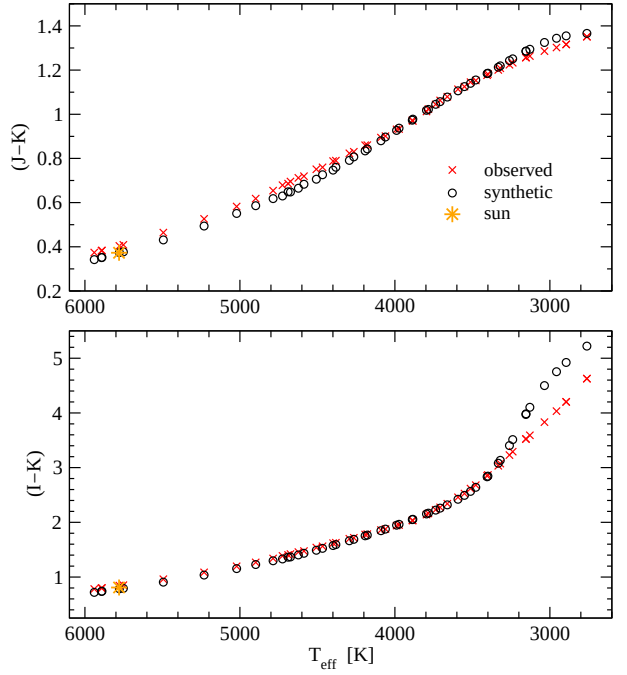
Figure 14. ( J-K ) and ( I-K ) as a function of the effective temperature for stars placed along an evolutionary track with one solar mass and Z/Z_{\odot} = 1.0 (see Fig. 4). The presented data and the plot symbols are the same as in Fig. 13
