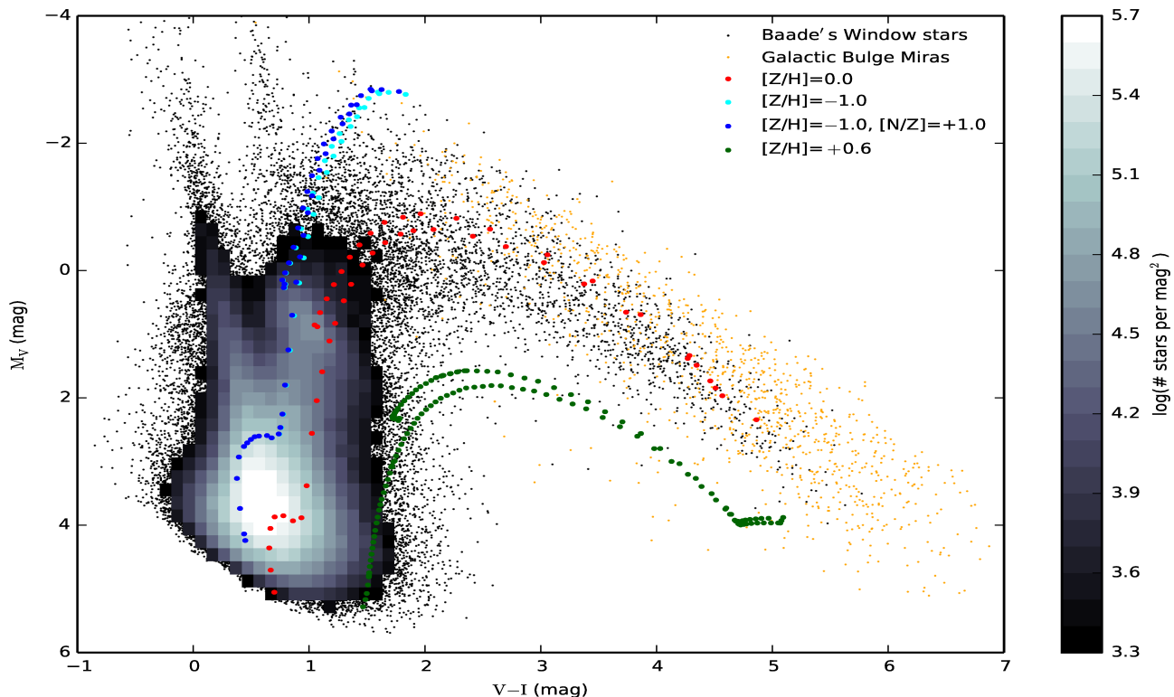
Figure 16. Colour-magnitude diagram M_V versus (V-I) for COMARCS models placed along evolutionary tracks for stars with one solar mass and Z/Z_\odot = 1.0 (red circles) as well as Z/Z_\odot = 0.1 (cyan circles). For the metal-poor track we show the effect of increasing nitrogen by a factor of ten ( [N/Z] = +1 , blue circles). The dots represent cool giants in Baade’s window (black) and Mira variables (orange) in the Galactic Bulge. Due to the large number of objects in the first group densities are plotted in the central region of their distribution. In addition, we show the points of a metal-rich evolutionary track with one solar mass and Z/Z_\odot = 3.98 (green circles), which were obtained from an interpolation in the COMARCS grid.
