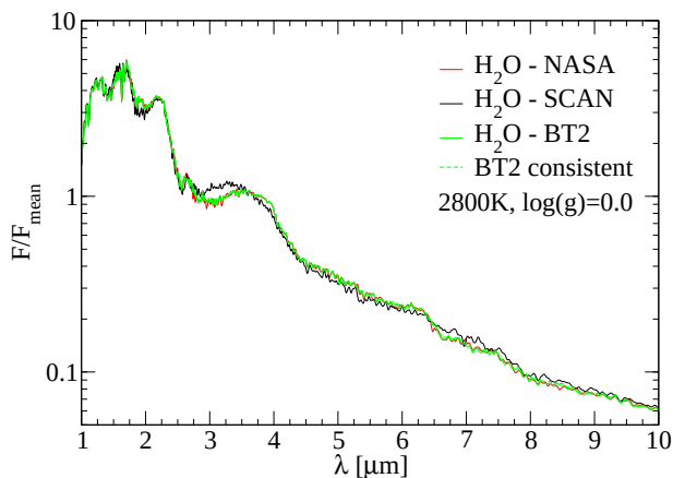
Figure 3. Spectra calculated with different \text{H}_2\text{O} data based on a COMARCS model with T_{\text{eff}} = 2800 K, \log(g [\text{cm/s}^2]) = 0.0 , one solar mass and solar metallicity. The SCAN (black, used in this work as standard), BT2 (green, used in this work as standard) and NASA-AMES (red) line lists are compared. The intensities \nu L_\nu are normalized to their mean value. We also show the result obtained with a consistent usage of the BT2 data for the computation of the atmospheric structure and the spectrum (green dashed), which is very similar to the one, where BT2 was only taken for the a posteriori radiative transfer (green full).
