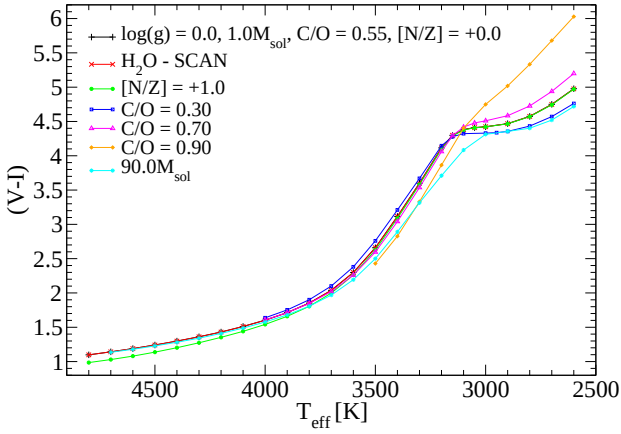
Figure 10. (V-I) as a function of the effective temperature for COMARCS models with solar metallicity and \log(g \text{ [cm/s}^2\text{]}) = 0.0 . Parameters, symbols and lines are like in Fig. 9.
