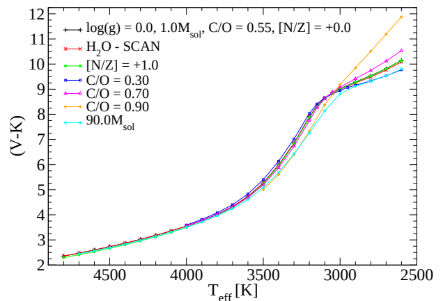
Figure 9. (V-K) as a function of the effective temperature for COMARCS models with solar metallicity and \log(g \text{ [cm/s}^2]) = 0.0 . The standard parameters are M/M_{\odot} = 1.0 , solar abundances ( \text{C}/\text{O} = 0.55 , [\text{N}/\text{Z}] = 0.0 ) and usage of the BT2 linelist for water below 4000 K (black). The result of changing C/O to 0.3 (blue), 0.7 (magenta) and 0.9 (orange), of increasing nitrogen by a factor of ten ( [\text{N}/\text{Z}] = +1.0 , green) or the mass to 90 M_{\odot} (cyan) is shown. In addition, we demonstrate the effect of taking the \text{H}_2\text{O} opacities from the SCAN data (red).
