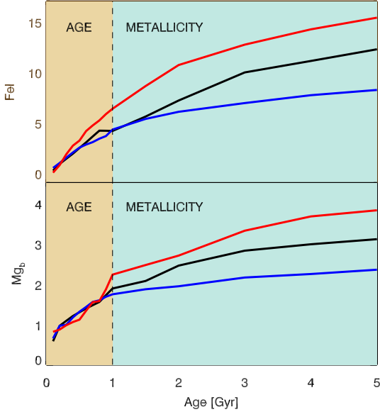
Figure 2. Examples of the different trends with age of two representative spectral indices, i.e. FeI(3000) and Mg_b , for MS11 and TMJ models respectively, for different stellar metallicities: sub-solar (blue lines), solar (black lines) and super-solar (red lines). For ages < 1 Gyr both indices are solid age -indicators, while for older ages they become better metallicity -indicators.
