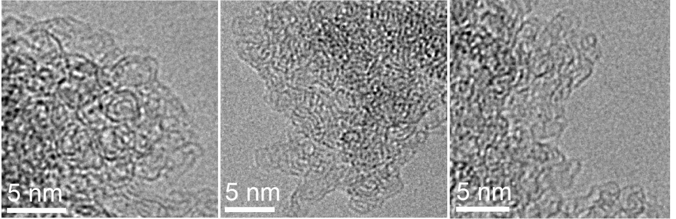
Fig. 9. Series of images presenting material with different levels of proton-induced processing. The three types of carbon structures were observed underneath the graphitic layer after complete bombardment of sample 3 with the total fluence of 6.76 \times 10^{16} ions/cm 2 . The particles are still visible, but they contain longer graphene layers compared to those observed in the original grains. In addition, one can see the formation of more closed buckyonions and fullerenes. The right micrograph finally shows grains, which are still similar to the unprocessed fullerene-like grains.
