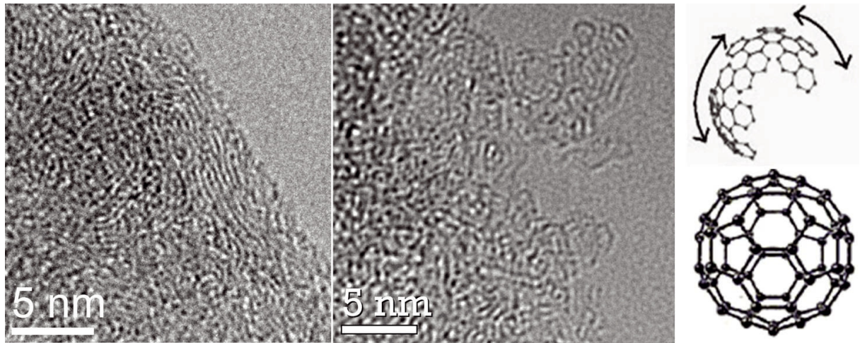
Fig. 10. Graphitic structures observed after bombardment of bare carbonaceous grains with 200 keV protons at total fluence of 6.76 \times 10^{16} ions/cm 2 (left). Fullerenes and bucky onions (middle), detected beneath the graphite layer, demonstrate the conversion of curved fullerene fragments into more closed structures (right).
