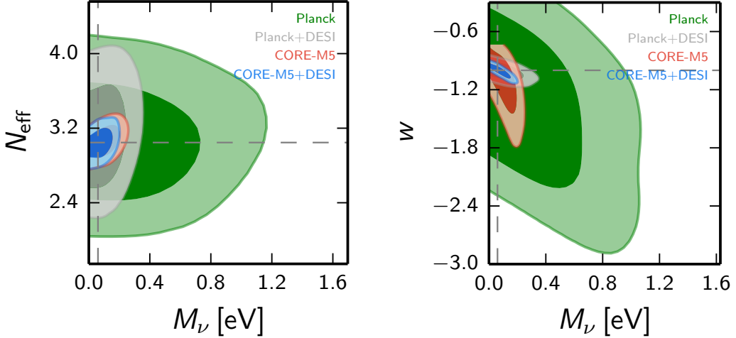
Figure 19. Constraints on the N_{\text{eff}} vs M_\nu plane (left panel) and w vs M_\nu plane (right panel) from Planck, Planck+DESI, CORE-M5, and CORE-M5+DESI simulated datasets. The dashed line corresponds to the \Lambda\text{CDM} prediction. \Lambda\text{CDM} with M_\nu = 0.06 eV is assumed as fiducial model.
