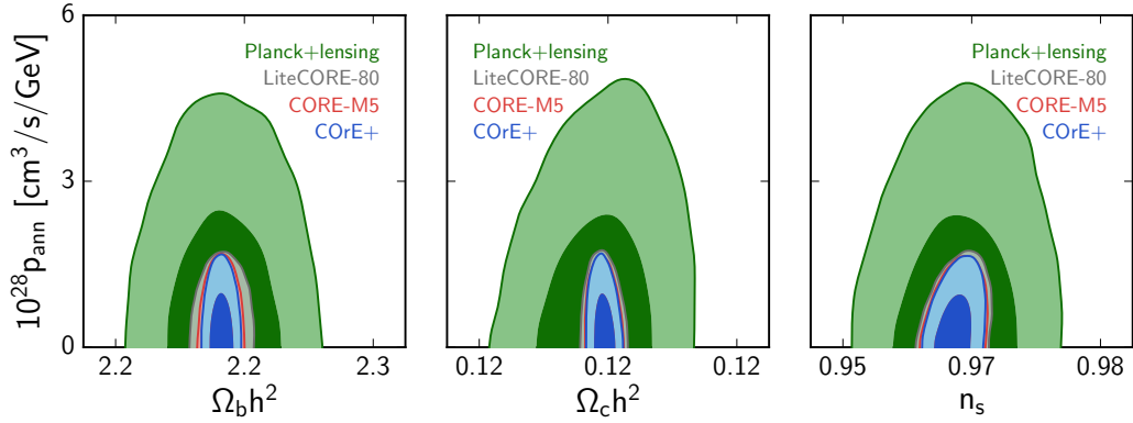
Figure 21. Results for the \Lambda\text{CDM} + p_{\text{ann}} model, showing some of the parameters most correlated with p_{\text{ann}} in the mock CORE data.
