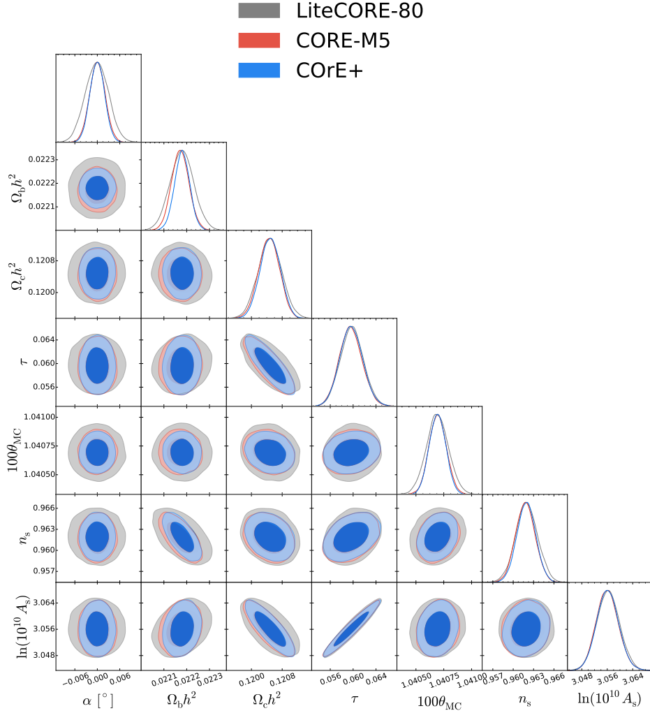
Figure 25. Triangular plot showing the main degeneracies between the comological parameters listed in table 33, for the three experimental configurations reported in this work.
