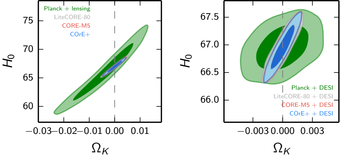
Figure 5. Left panel: constraints on the H_0 vs \Omega_k plane from different CORE configurations. Current constraints from Planck+CMB lensing are reported for comparison. Right panel: constraints on the H_0 vs \Omega_k plane for the following (simulated) datasets: Planck+DESI, LiteCORE80+DESI, CORE-M5+DESI, CORE++DESI. A flat universe is assumed in the simulated data.
