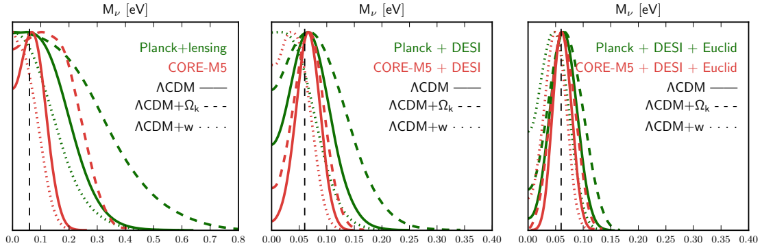
Figure 11. Posterior distribution of the summed neutrino mass in the extended models \Lambda\text{CDM} + M_\nu , \Lambda\text{CDM} + M_\nu + w and \Lambda\text{CDM} + M_\nu + \Omega_k . The vertical dashed line shows the fiducial value.
