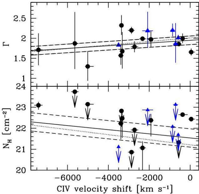
Fig. 3. \Gamma and N_{\text{H}} as a function of v_{\text{CIV}} (top and bottom panels). The meaning of the data points and linear fits is the same as in Fig. 1.
