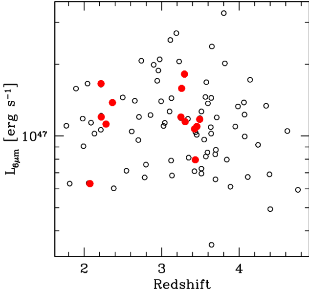
Fig. A.1. L_{6\mu\text{m}} versus z for our WISSH sub-sample (filled red circles) and the entire WISSH sample (empty black circles).
