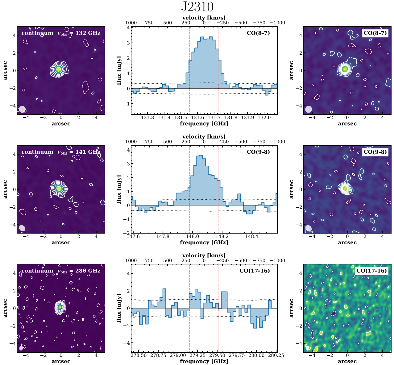
Figure 1. J2310. Left-hand panels: continuum emission maps at 132 GHz (top), 141 GHz (middle), and 280 GHz (bottom). Contours are plotted at levels of (-2, 2, 4, 8, 16, 32, 64) times \sigma . The rms noise level is 15, 15, and 42 \mu\text{Jy beam}^{-1} , respectively, for the three maps. In each map, the ALMA beam is plotted on the bottom left-hand corner. Central panels: continuum subtracted spectra extracted from a region of radius 1.5 arcsec. From top to bottom we report the spectrum of CO(8–7), CO(9–8), and CO(17–16). All spectra are rebinned at the same spectral resolution of 40 \text{km s}^{-1} and the horizontal dotted lines indicate the noise level as a function of frequency. Vertical dashed red lines represent the frequency/velocity range used to extract the flux map shown in the right-hand panels. Right-hand panels: flux maps of CO(8–7) (top), CO(9–8) (middle), and CO(17–16) (bottom). Emission is integrated in channels with |v| < 200 \text{ km s}^{-1} relative to the frequency of the CO lines. Contours are shown in step of 2\sigma starting from \pm 2\sigma , where 1\sigma is 40, 40, and 70 \text{mJy beam}^{-1} \text{ km s}^{-1} , respectively, for the three molecular lines.
