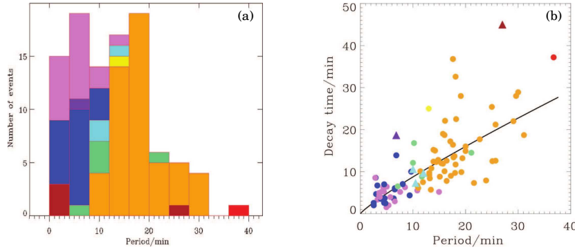
Fig. 6 Physical properties of observed slow-mode oscillations (from Nakariakov et al., 2019b). (a) Distribution of the wave periods for different detection temperatures. (b) Scaling of the damping time with the period. In (a) and (b) the colors represent different temperatures: violet for 14 MK, magenta for 13 MK, blue for 12 MK, cyan to 10 MK, green for 8.9 MK, yellow for 7 MK, orange to 6.3 MK, red to 2 MK, and brick for 0.6 MK. In (b) the circles show SUMER and BCS oscillations and triangles show AIA oscillations. The black line indicates the best-fitting power law.
