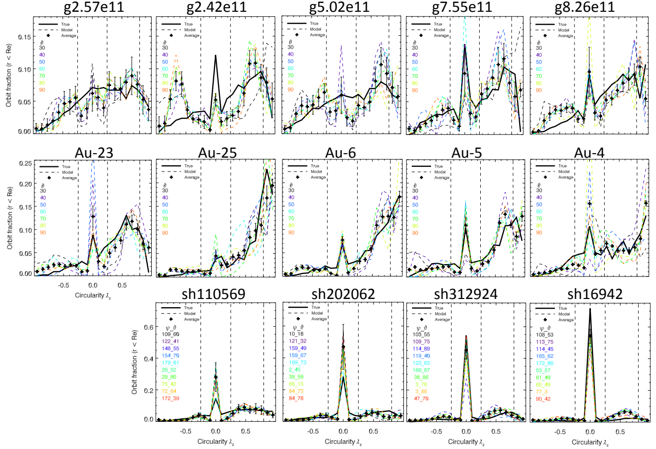
Figure 6: Supplementary Figure 2: Orbital circularity \lambda_z distribution within R_e for 14 of the 15 simulated galaxies (similar figure for S_1 in Zhu et al. 2017a). In each panel, the true \lambda_z distribution of the simulated galaxy is shown as the black solid line. Each coloured line is the average orbital distribution from modelling a mock data set with viewing angles as labeled. The error bars show the typical 1\sigma scatter for each mock data set. Crosses denote the average of the seven/ten different dashed lines for spiral/elliptical galaxies.
