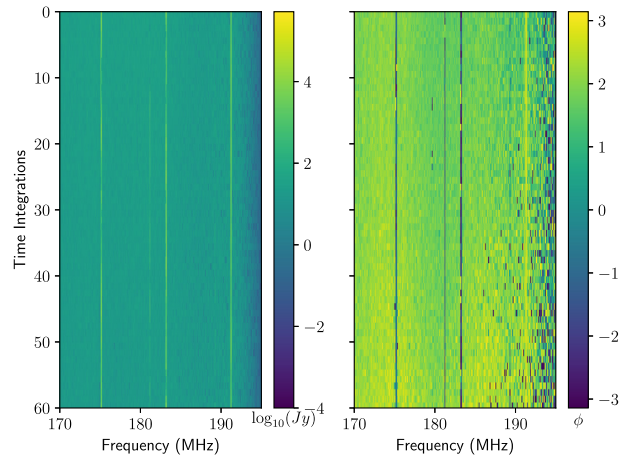
Figure 1. An example of a HERA 14 m baseline waterfall visibility between 170 and 195 MHz in amplitude (left) and phase (right). The phase waterfall visibility demonstrates how it can provide complementary information about the presence of RFI such as in the 181.3 MHz channel which has constant narrow-band RFI and the more spontaneous ‘blips’ in the 179.5 MHz channel at time integrations of 13, 22, and 23. The significant contrast between the phase of the sky fringe, and how it is restricted to a narrow band is an obvious indication of being RFI.
