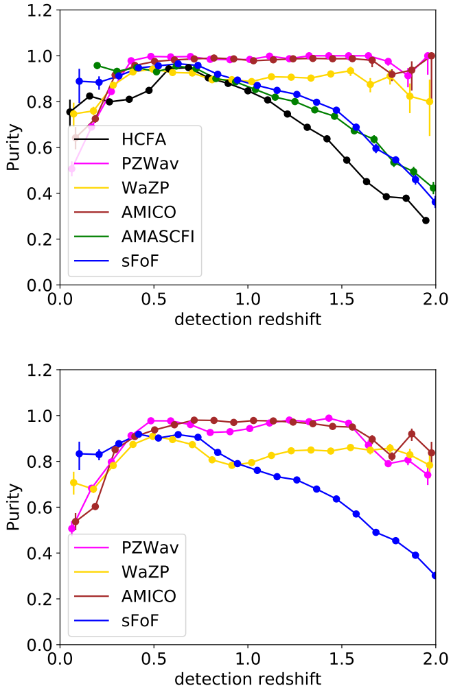
Fig. 12. Purity as a function of redshift for a mean completeness of the detection catalogs set to 65% ( top panel ) and 80% ( bottom panel ) in the range 0 < z_{\text{true}} < 2 and for masses M > 10^{14} M_{\odot} . AMASCFI and HCFA do not reach the 80% completeness level and are thus not represented in the bottom panel. Error bars are computed as in Fig. 11.
