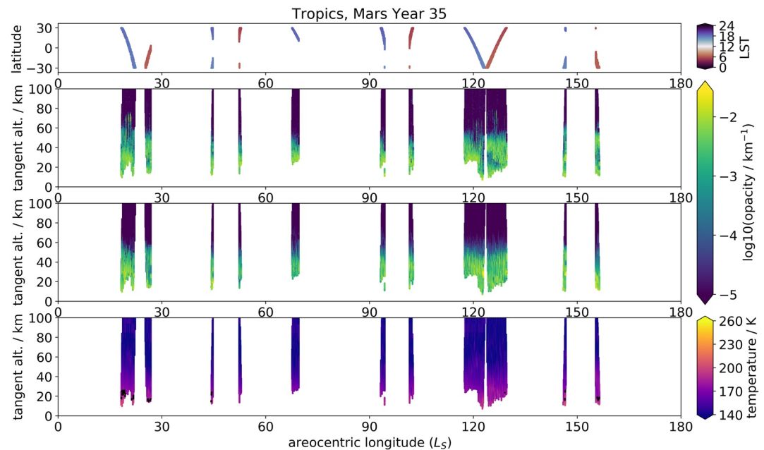
Figure 4. Same as Figure 3, absent the 600/320 ratios and filtered to only include tropical latitudes from L_S = 0^\circ – 180^\circ .
