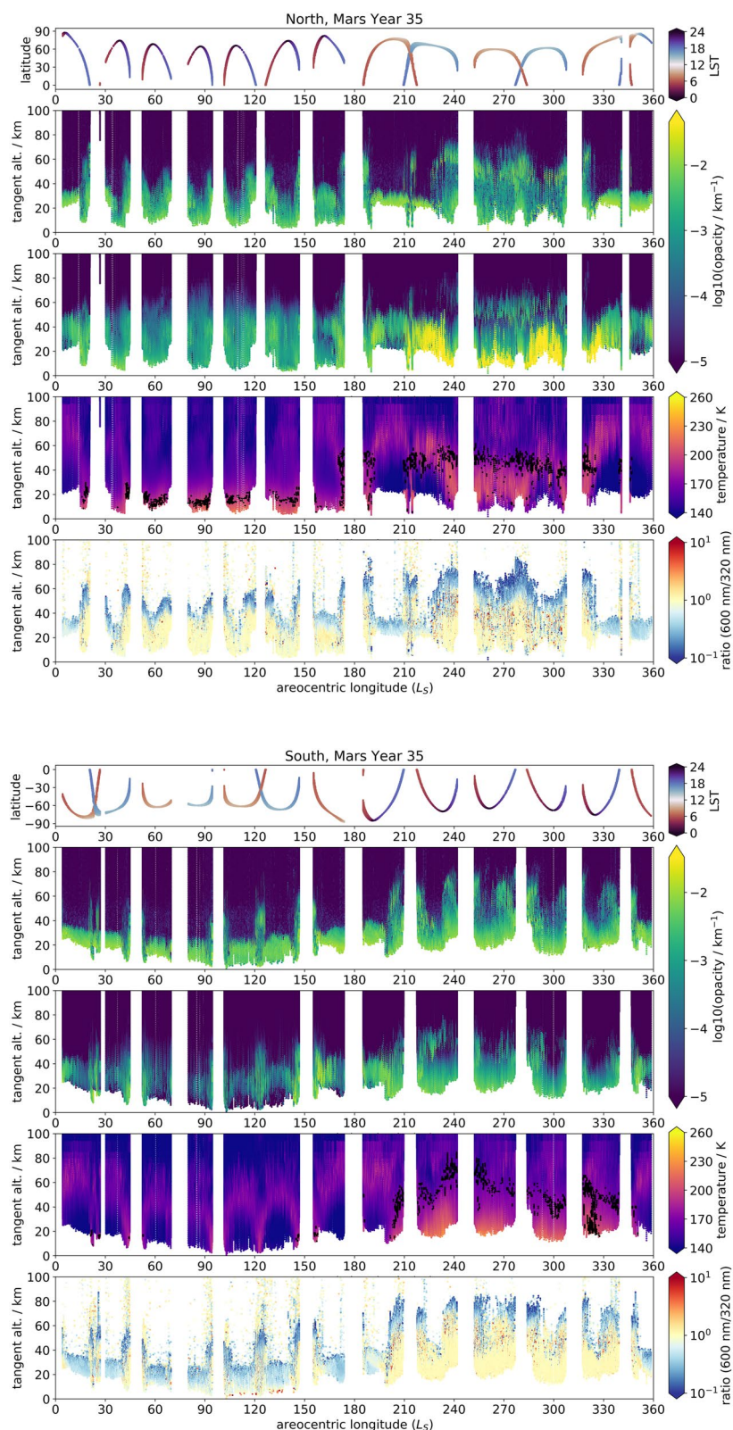
Figure 3. Same as Figure 2 for MY 35.
