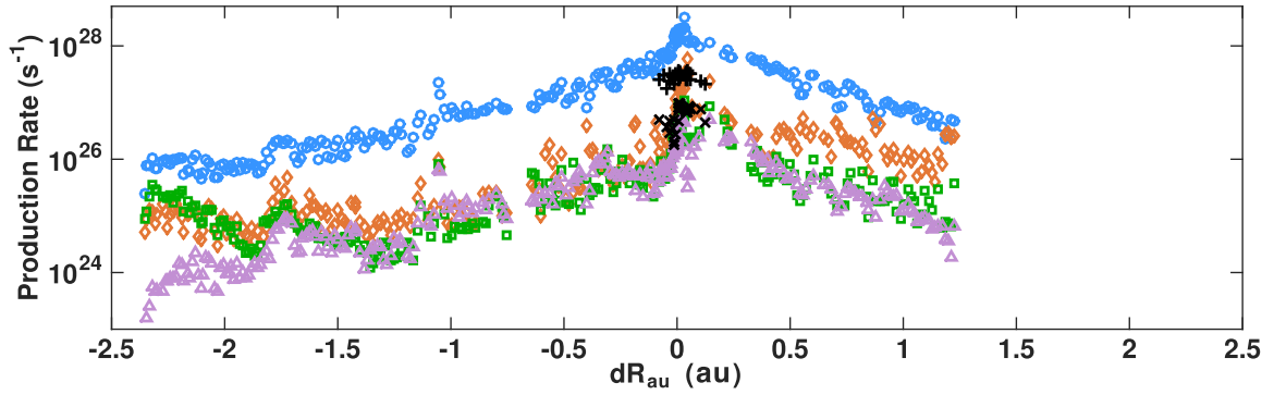
Figure 11. Evolution of the production rate for the species H 2 O (blue), CO 2 (orange), CO (green), and O 2 (purple) from the DFMS data using the DSMC model to take into account the asymmetry of the coma and the evolution of the velocity as a function of heliocentric distance with respect to the closest approach (1.24 au) dR_{\text{au}} using the definition that dR_{\text{au}} is negative before perihelion and positive after perihelion. The black plus and cross symbols represent, respectively, the H 2 O and CO 2 production rates deduced from the VIRTIS-H observations using the DSMC model.
