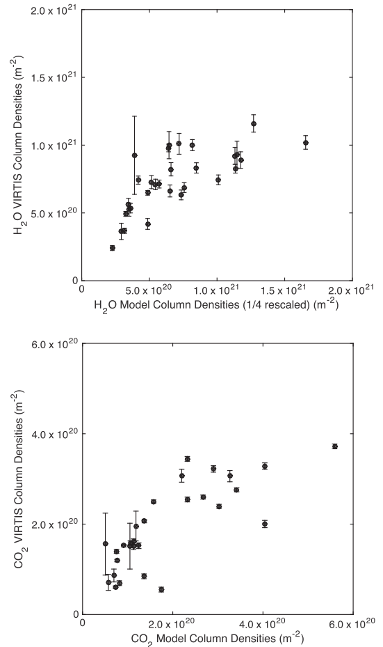
Figure 10. VIRTIS-H column densities deduced from observation times ranging from 2015 July 8 to 2015 September 27 (Bockelée-Morvan et al. 2016) as a function of the model column densities for \text{H}_2\text{O} and \text{CO}_2 . The model \text{H}_2\text{O} column densities were applied a factor of 0.25 to match the data range.
