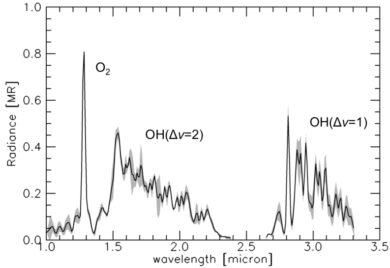
Figure1. VIRTIS mean nightglow spectral radiance, in the altitude range 87-105 km. This dataset was processed with a median filter applied to the spatial component, in order to eliminate instrumental artifacts and with a background correction obtained by subtracting the spectrum measured between 120 and 125 km. Finally a wavelength calibration adjustment has been performed by applying a shift of \sim 11 nm towards shorter wavelengths (see also Migliorini et al. [2013]). The shaded area indicates the experimental error, calculated from the Noise Equivalent Spectral Radiance (NESR). The O_2 and OH(\Delta v=1,2) emissions are indicated.
