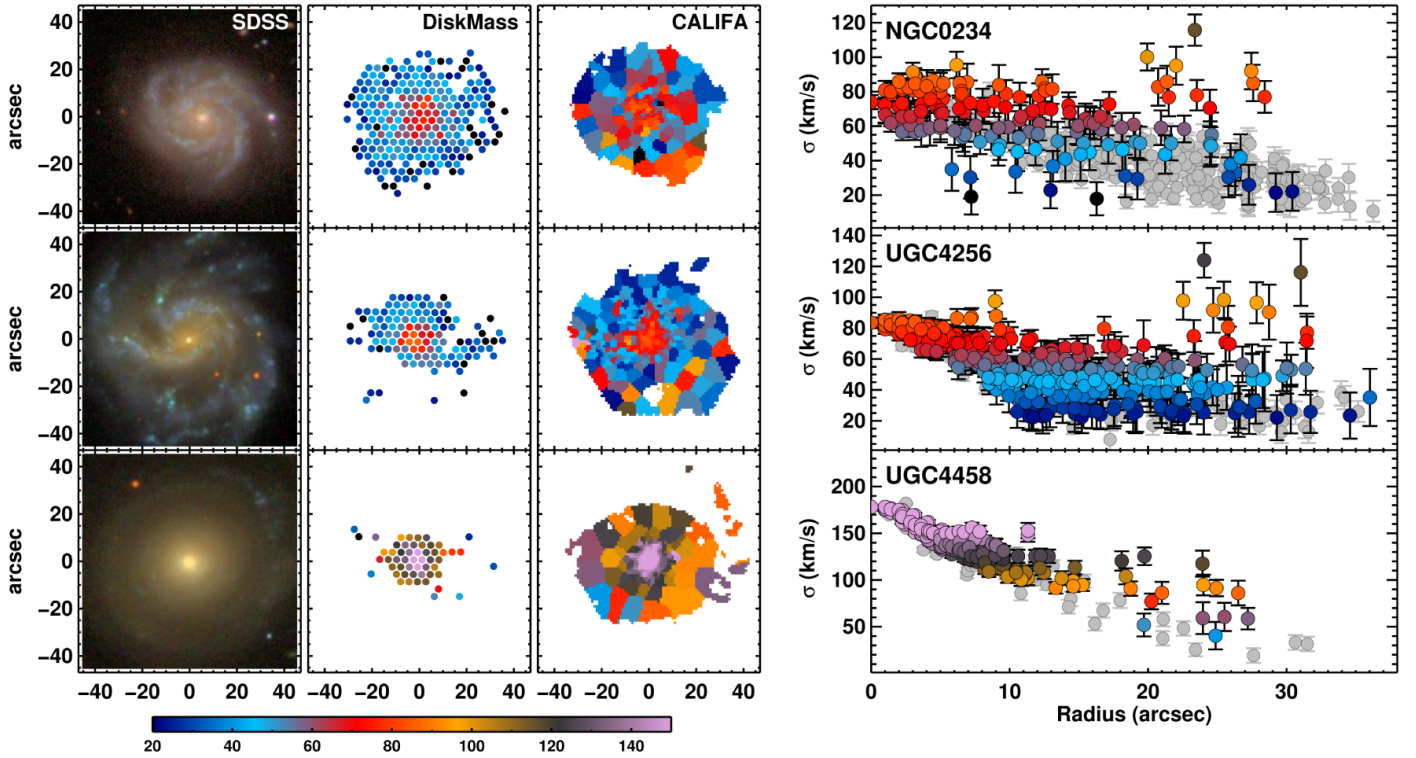
Fig. 8. Comparison of the stellar velocity dispersion maps and radial profiles from the CALIFA and DiskMass surveys. Each row shows (from left to right): a color-composite SDSS image of the galaxy, the DiskMass velocity dispersion map (see Sect. 5 for details), the CALIFA velocity dispersion map, and the radial velocity dispersion profile (extracted in circular annuli). DiskMass measurements are in gray while the CALIFA measurements are in color following the same color scheme of the maps (also indicated with the colorbar below). Empty (i.e., white) regions within some of the CALIFA maps are areas masked during our kinematic extraction. All velocity dispersion measurements are expressed in \text{km s}^{-1} .
