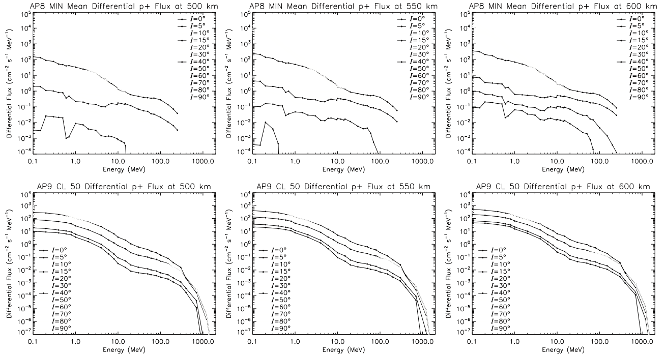
Figure 4. Orbit averaged differential fluxes of trapped protons for mean AP8 MIN (top panels) and AP9 50% CL (bottom panels) models computed for altitudes 500, 550 and 600km altitudes, respectively, from left to right and for different orbital inclinations I .
