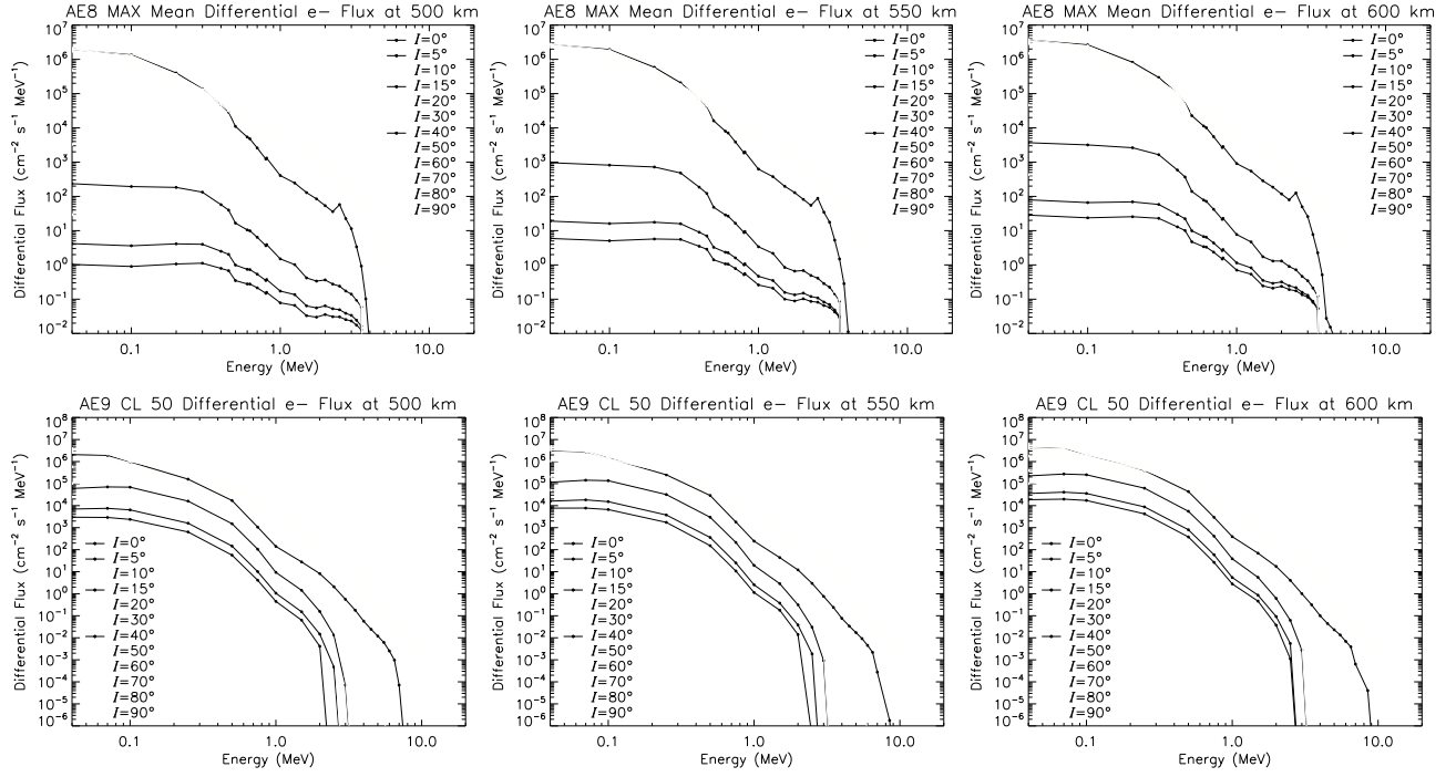
Figure 3. Orbit averaged differential fluxes of trapped electrons for mean AE8 MAX (top panels) and AE9 50% CL (bottom panels) models computed for altitudes 500, 550 and 600km altitudes, respectively, from left to right and for different orbital inclinations I .
