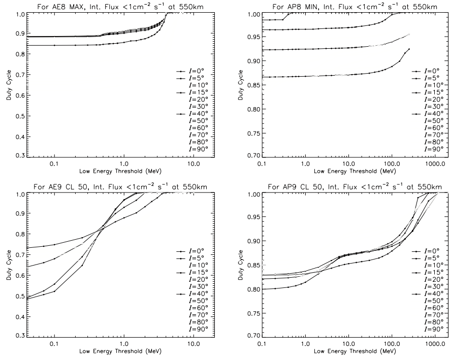
Figure 9. Duty cycle for particle flux < 1 \text{ cm}^{-2} \text{ s}^{-1} for different orbital inclination as a function of the low-energy threshold for AE8MAX (top left), AE9 50 % CL (bottom left) models of trapped e^- and AP8MIN (top right), AP9 50 % CL (bottom right) models of trapped p^+ .
