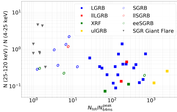
Fig. 8 Hardness ratio N(25-120 \text{ keV}) / N(4-25 \text{ keV}) as a function of the ratio N_{\text{tot}} / N_{\text{peak}_{64\text{ms}}} in the 4-120 keV energy range.
