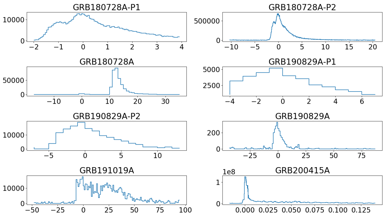
Fig. 11 light curves used to simulate the photon counts from GRBs in the movegrb-simulator program. The x-axis is in s while the y-axis is the expected cnt/ s per bin.
