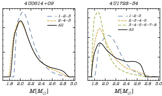
FIG. 6.— Posterior distributions for the mass of the binary systems 4U0614+09 and 4U1728-34. Dashed curves refer to different grouping of kHz QPO doublets, whereas the solid black lines are obtained by fitting all doublets for each source.
