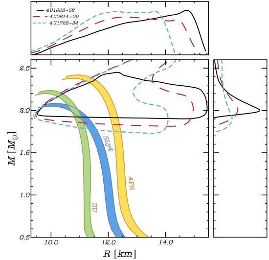
FIG. 7.— 90% 2D credible interval and marginalised distributions of the mass and radius for the 3 sources analysed. Colored curves are from of a few EoS whose M - R relation is compatible with current constraints from X-ray observations and the gravitational-wave event GW170817. The left and right edges of each colored band correspond to stellar configurations for which the spins are assumed to be zero and equal to the median of the values inferred by our MCMC analysis, respectively.
