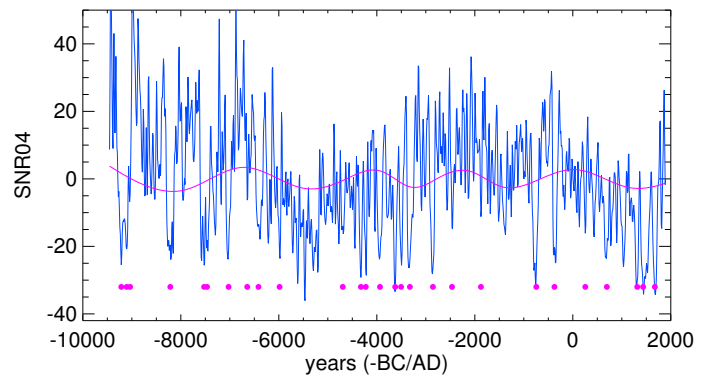
Fig. 11. Intrinsic mode function \psi_0 (magenta line), associated with the Hallstatt cycle, superimposed onto the sunspot number SNR04 dataset (blue line). Magenta dots correspond to the grand minima identified in this paper.
