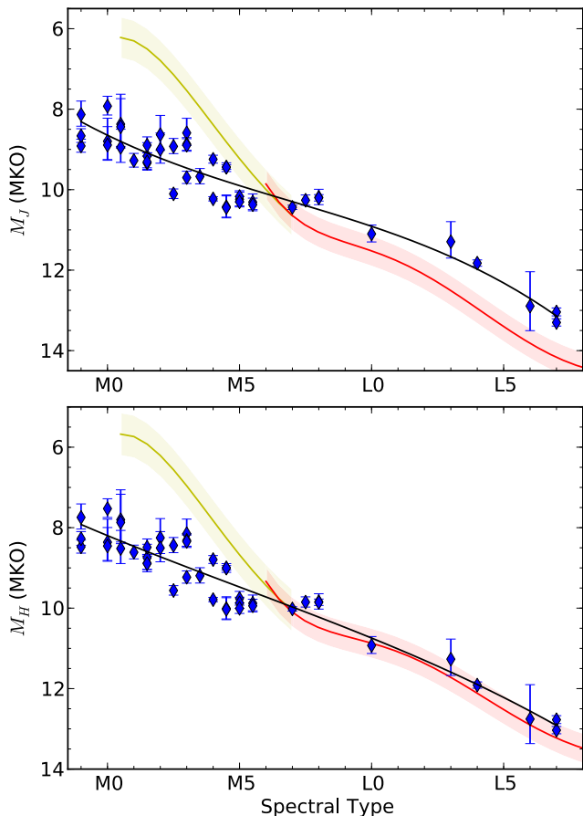
Figure 16. Relationships of spectral types and J - and H -band absolute magnitudes of M and L dwarfs updated from Zhang et al. (2013), which are plotted as black lines in both panels. The relationships for M0.5–M7 dwarfs (yellow lines) from Zhang et al. (2013) and M6–L dwarfs (red lines) from Dupuy & Liu (2012) are plotted for comparison. Shaded areas show their fitting rms.
