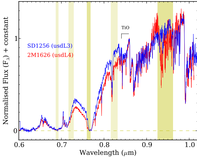
Figure 12. Optical spectra of SD1256 and 2M1626. Spectra are normalized at 0.86 \mu\text{m} . Telluric absorptions are corrected.
