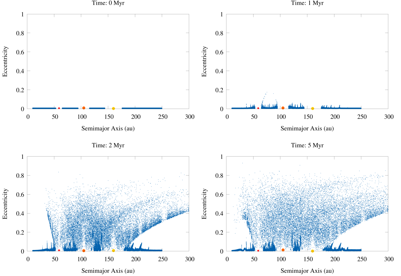
Figure 3. Temporal evolution, in the semimajor axis–eccentricity plane, of the dynamical state of the planetesimal disk of HD 163296 in our reference scenario (i.e planetary masses as estimated by Liu et al. 2018). Going from left to right, top to bottom, the panels show the evolution from the initial state of the planetesimal disk in our simulations (top left panel) to its potential current state (bottom right panel).
