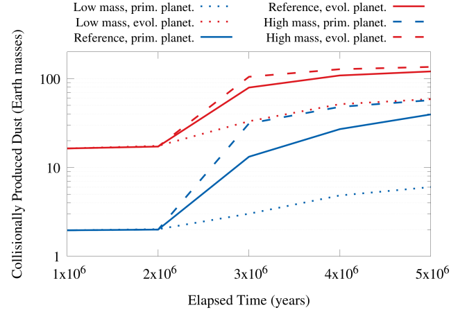
Figure 7. Comparison between the global dust production (in M_{\oplus} ) of the planetesimal collisional evolution over each 1 Myr of life of HD163296’s system in the three scenarios for the planetary masses (“low mass” scenario: dotted lines; reference scenario: solid line; “high mass” scenario: dashed line) and for the two size-frequency distributions of the planetesimals we considered (primordial size-frequency distribution: blue line; collisionally evolved size-frequency distribution: red line).
