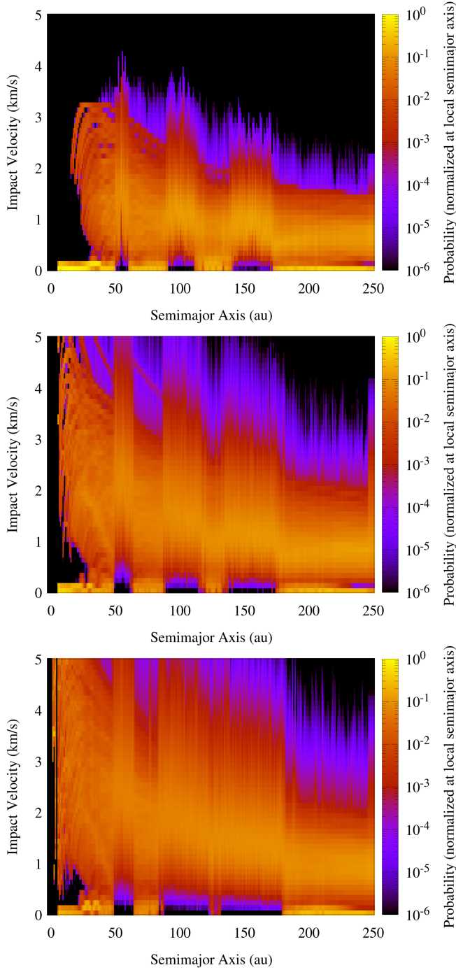
Figure 6. Comparison of the impact velocities across the planetesimal disk of HD 163296 at 5 Myr in the three scenarios we considered for the mass values of the giant planets. From top to bottom the plots show the “low mass” scenario (planets possessing the mass values estimated by Isella et al. 2016 ), the reference scenario (planets possessing the mass values estimated by Liu et al. 2018 ), and the “high mass” scenario (the two outer planets possessing the mass values estimated by Teague et al. 2018 ). The color code indicates the probability distribution of the impact velocities normalized at the local semimajor axis. This means that that each vertical slice of the plot represents the impact velocity distribution for planetesimals at that specific semimajor axis.
