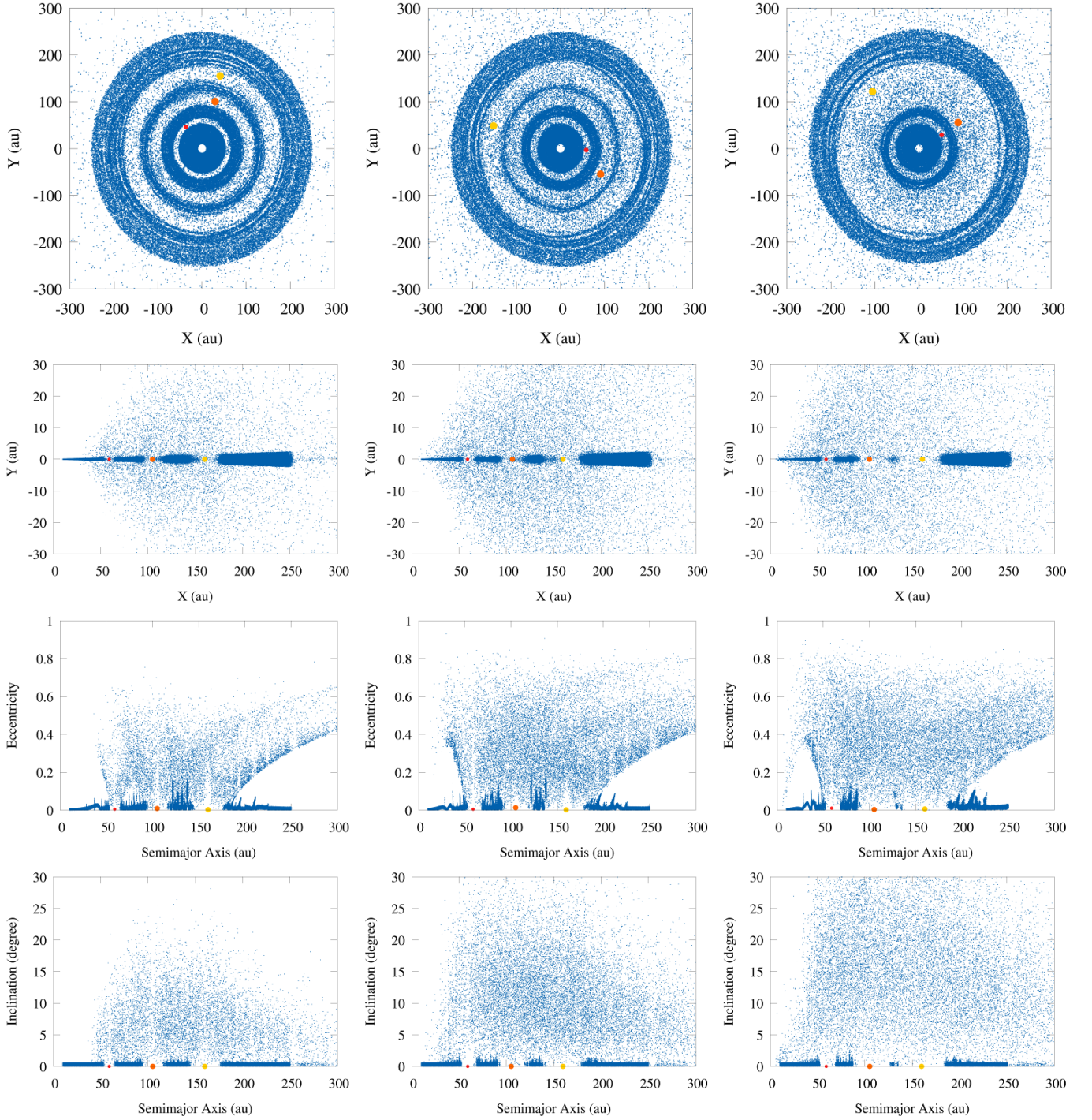
Figure 5. Comparison of the orbital structure and dynamical excitation of HD 163296’s planetesimal population at 5 Myr in the three scenarios we considered for the mass values of the giant planets. From left to right, the plots show the “low mass” scenario (planets possessing the mass values estimated by Isella et al. 2016 ), the reference scenario (planets possessing the mass values estimated by Liu et al. 2018 ), and the “high mass” scenario (the two outer planets possessing the mass values estimated by Teague et al. 2018 ). From top to bottom, the plots show the disk of planetesimals seen “face on” and “edge on”, the disk of planetesimals in the semimajor axis–eccentricity plane, and the disk of planetesimals in the semimajor axis–inclination plane.
