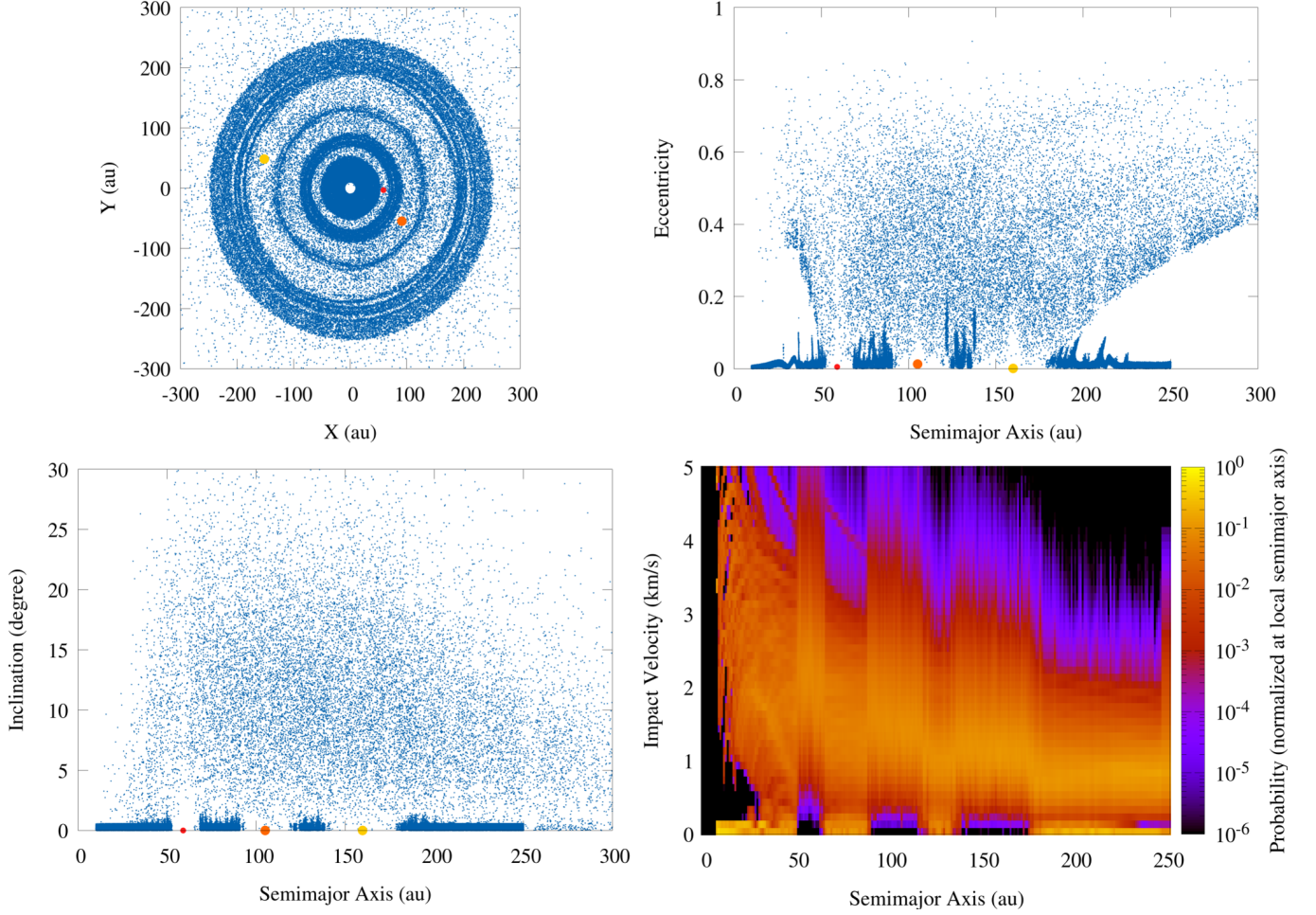
Figure 2. Dynamical state of the planetesimal disk of HD 163296 in our reference case (i.e. planetary masses as estimated by Liu et al. 2018) after 5 Myr due to the excitation caused by its three giant planets. Top left: “face-on” orbital structure of the planetesimal disk. Top right: orbital eccentricities of the planetesimals in the excited circumstellar disk. Bottom left: orbital inclinations of the planetesimals in the excited circumstellar disk. Bottom right: radial distribution of the impact velocities among planetesimals throughout the excited circumstellar disk. The color code indicates the probability distribution of the impact velocities normalized at the local semimajor axis. This means that each vertical slice of the plot represents the impact velocity distribution for planetesimals at that specific semimajor axis.
