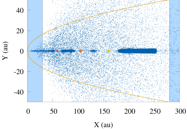
Figure 9. “Edge-on” view of the planetesimal disk at 5 Myr in the “high mass” scenario (inner planet with the mass value estimated by Liu et al. 2018 , outer two planets possessing the mass values estimated by Teague et al. 2018 ). The two continuous lines indicate the locations of the geometrically thin layers responsible for the CO thermal emission identified by Isella et al. (2018) . The two highlighted areas between 0 and 30 au and beyond 280 au are those where the measured temperatures are significantly lower than those predicted by fitting models of the CO-emitting layers and they coincide with the regions where the CO-emitting region is not crossed by supersonic planetesimals (0-30 au) and where the spatial density of supersonic planetesimals drops significantly (>280 au).
