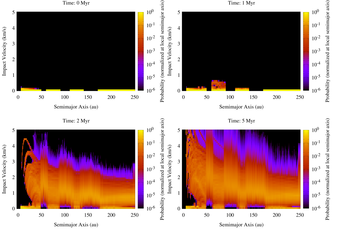
Figure 4. Temporal evolution of the impact velocities across the planetesimal disk of HD 163296 in our reference scenario (i.e. planetary masses as estimated by Liu et al. 2018). Going from left to right, top to bottom, the panels show the evolution of the impact velocity distribution from the initial state of the planetesimal disk in our simulations (top left panel) to its potential current state (bottom right panel). The color code indicates the probability distribution of the impact velocities normalized at the local semimajor axis. This means that that each vertical slice of the plot represents the impact velocity distribution for planetesimals at that specific semimajor axis.
