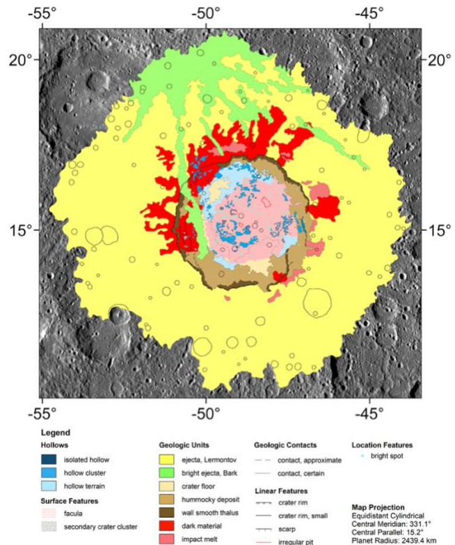
Figure 1: Geological map of Lermontov crater.
