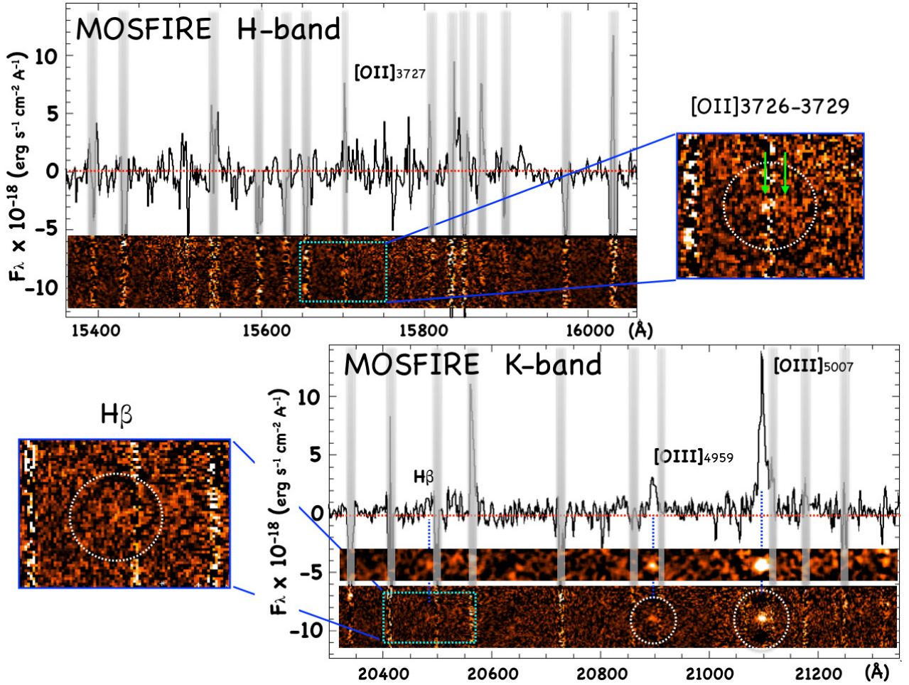
Fig. 4. Two- and one-dimensional near-infrared spectra of Ion2 in the MOSFIRE H - and K -band. Two insets show the regions where H \beta and the [O II]λ3727 doublet are expected from the redshift. The gray stripes in the one-dimensional spectra indicate the position of the sky lines.
