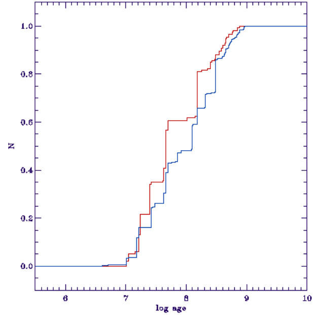
Fig. 8. Cumulative distribution of log(age) for the stars in our sample (red line) and that of Nielsen et al. (2019) (blue line).
