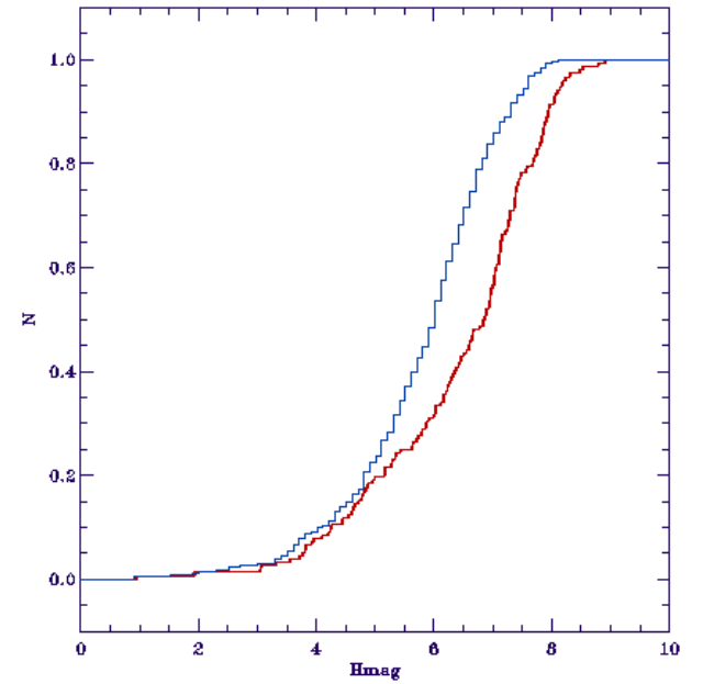
Fig. 5. Cumulative distribution of H -band magnitude for the stars in our sample (red line) and that of Nielsen et al. (2019) (blue line).
