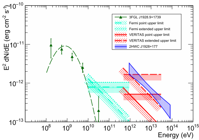
Figure 5. SED of 2HWC J1928+177. The blue solid area shows the 1 \sigma confidence interval of HAWC’s spectrum measurements. The solid red lines show the VERITAS upper limits from the point-source search, assuming either the spectral index measured by HAWC or a spectral index of 2. The dashed red lines show the VERITAS upper limits from the extended-source search for the same spectral indices. The corresponding Fermi -LAT upper limits are shown as teal dot-dashed lines for the point-source search and teal dashed lines for the extended-source search. The green triangle points and dashed line show the flux of the nearby 3FGL source, 3FGL J1928.9+1739.
