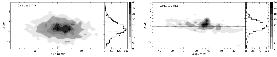
Figure 10. A comparison of GALAH radial velocities with values from RAVE (left-hand panel) and APOGEE (right-hand panel). The x-axis is the GALAH radial velocity in \text{km s}^{-1} while the y-axis is the difference between the GALAH value and that from the other survey, in the sense (GALAH–other). Colour, as denoted by the bar, indicates the number density of stars. The right-hand portion of each figure shows the distribution of the difference in radial velocity. The top-left corner lists the mean and standard deviation in radial-velocity difference.
