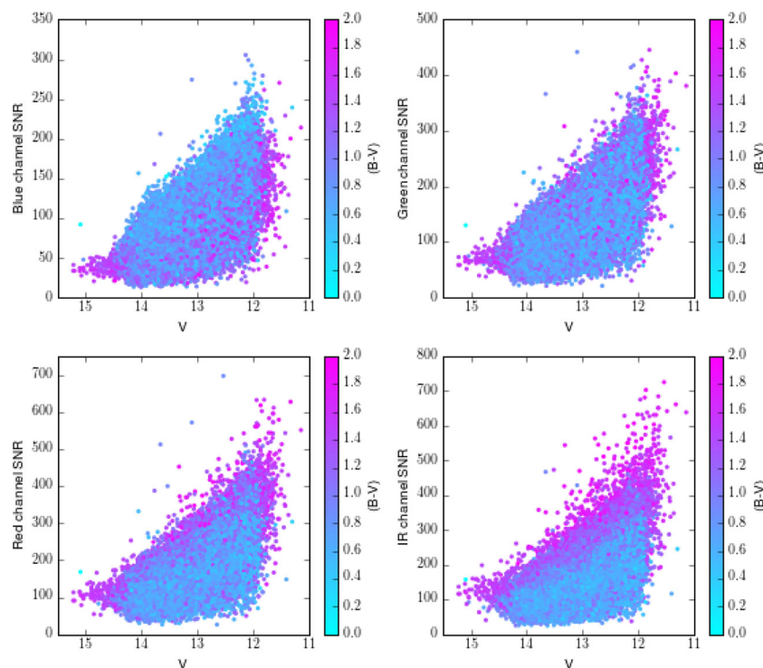
Figure 4. SNR per resolution element for all four HERMES channels versus apparent V magnitude for the example data set, colour-coded by (B - V) colour. Blue stars have higher blue channel SNR, but their SNR drops relative to the redder stars in the redder channels.
