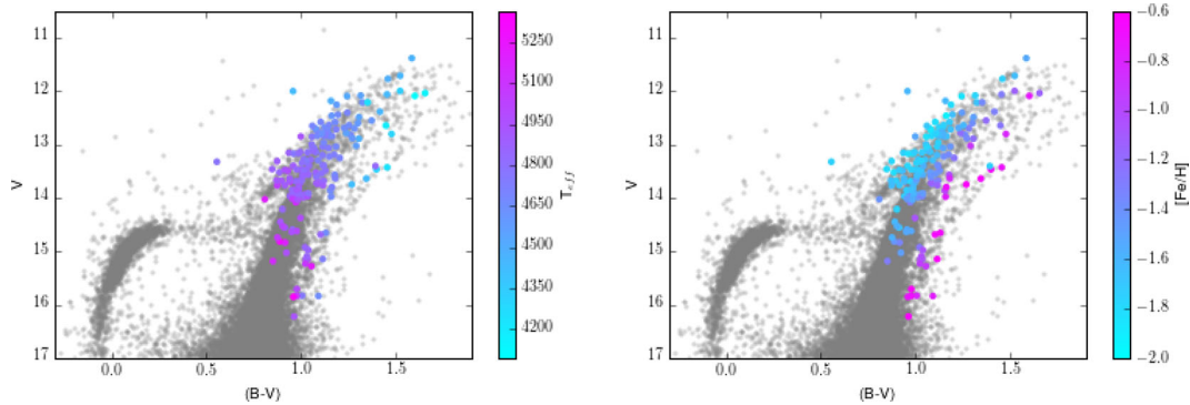
Figure 6. The (V, B - V) colour–magnitude diagram for \omega Centauri, colour-coded by GALAH effective temperature (left-hand panel) and metallicity (right-hand panel). All stars within 10 arcmin of the cluster centre, with membership probability from Bellini et al. (2010) above 0.9, are shown as smaller grey circles. Both T_{\text{eff}} and [\text{Fe}/\text{H}] behave as expected, both in terms of range and trends.
