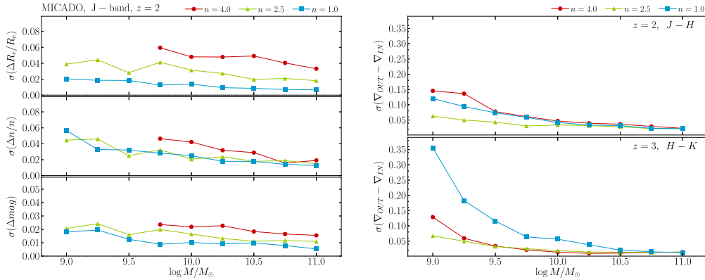
Figure 1. Left panel: Uncertainty on the effective radius, Sersic index ( n ), and total magnitude obtained from simulated MICADO@E-ELT observations in the J -band of galaxies at z = 2 with various morphology. Right panel: Uncertainty on the color gradient ( J-H and H-K ) measured on galaxies at redshift 2 and 3.
