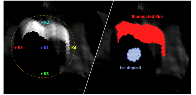
Figure 9. Simulated illumination conditions, or \cos(i) , occurring on Kandinsky crater at TA = 200^\circ (left-hand panel). The area of the sun illuminated rim (in red, departing from point K2) and the location of the putative water ice deposit (the blue dots, corresponding to location K1) on the unilluminated crater floor are shown on the right-hand panel.
