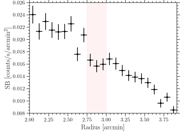
Figure 8. In the XMM-Newton image on the left panel we report the sector used to extract the X-ray surface brightness profile shown in the right panel. Inner ticks in the sector mark the radial range highlighted in the profile that may exhibit a surface brightness dip. Radio contours are the same of Fig. 4.
