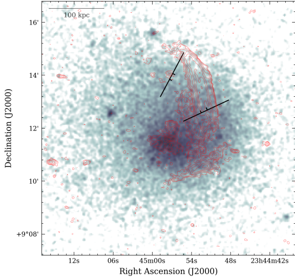
Figure 8. In the XMM-Newton image on the left panel we report the sector used to extract the X-ray surface brightness profile shown in the right panel. Inner ticks in the sector mark the radial range highlighted in the profile that may exhibit a surface brightness dip. Radio contours are the same of Fig. 4.
