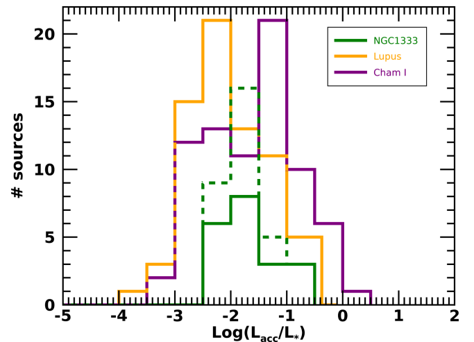
Fig. 8: Histograms of the luminosity ratio L_{\text{acc}}/L_{\star} of NGC 1333, Lupus, and Cha I samples are shown in green, orange, and purple, respectively. The green-dashed line corresponds to the histogram of NGC 1333, including the upper limits.
