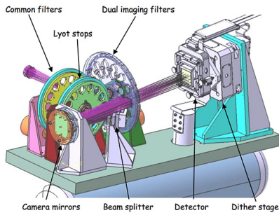
Fig. 19: IRDIS opto-mechanical layout (left), and picture of the IRDIS cryostat during integrations (right).
