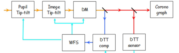
Fig. 4: Block diagram of the AO components and loops in SPHERE. As in Fig. 1, VIS+NIR light is in orange, VIS light is in blue and NIR light is in red. The control loops are in light-blue.
