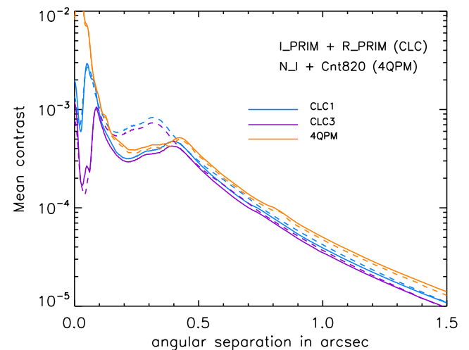
Fig. 12: Visible normalized contrast for several coronagraphic configurations of ZIMPOL, as measured on 9 October 2014 on HR 591.
