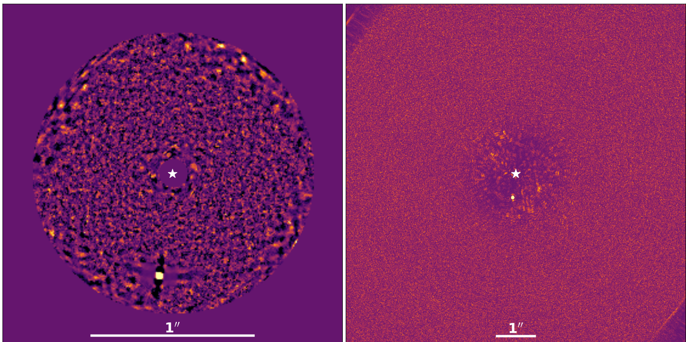
Fig. 20: Example of IFS (Y-J, left) and IRDIS (H2 filter, right) images of the spectro-photometric calibrator HD 114174 obtained by using in ADI for 1 h observing time. The IRDIS images are processed with cADI, while the IFS ones are processed with ASDI PCA.
