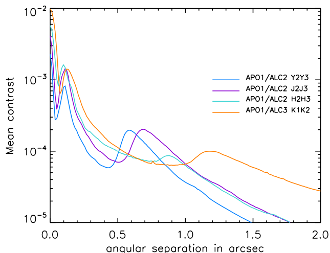
Fig. 9: Near-infrared normalized contrast for two coronagraphic configurations (APO1/ALC2 and APO1/ALC3) in different filter pairs (Y23, J23, H23, K12) as measured on 15 May 2014 on HD 140573.
