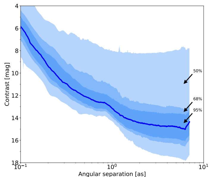
Fig. 22: Median 5\sigma contrast achieved by IRDIS in DBI H23 mode (H2 ADI only) in 1h30 observing time on average with T-LOCI post-processing. The plain blue line represents the median, and the different shades of blue background represent the 95%, 68% and 50% completeness intervals.
