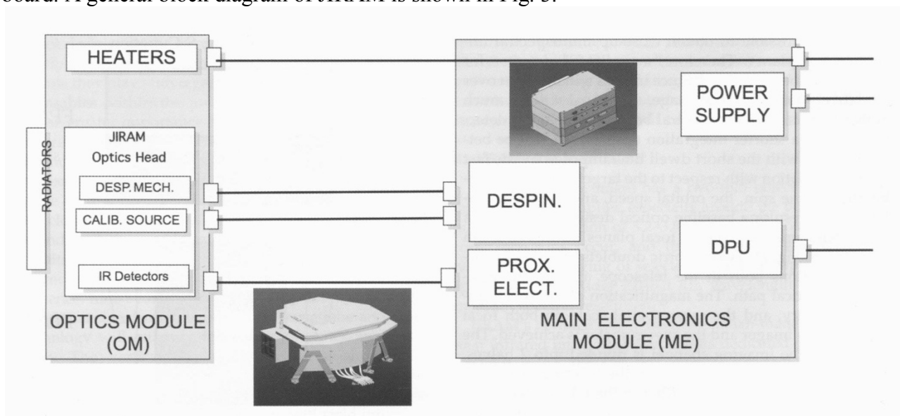
Figure 4: General block diagram of JIRAM.
