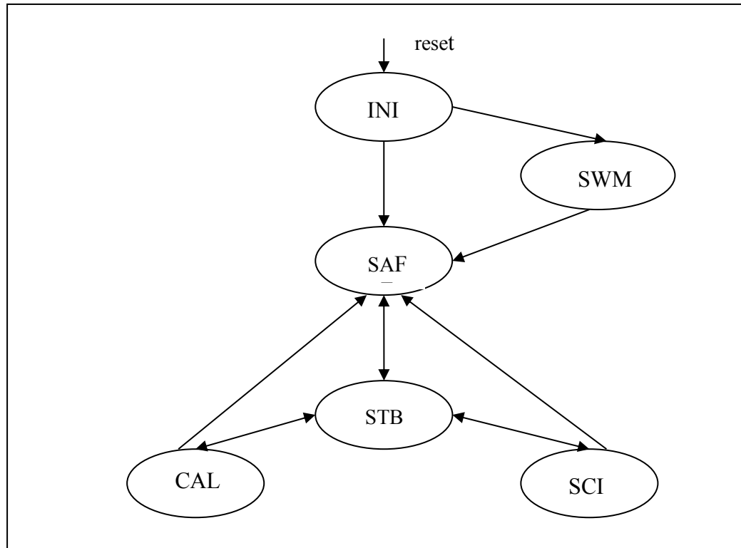
Figure 5: JIRAM FSW modes
