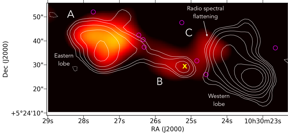
Fig. 5. Diffuse X-ray emission (components A, B, and C) as seen by Chandra in the full 0.5–7 keV band with LOFAR 144-MHz contours overlaid in white (same as Fig. 2). The protocol cluster galaxy members as reported in Fig. 1 are marked with magenta circles, and the radio galaxy host is marked with a yellow cross.
