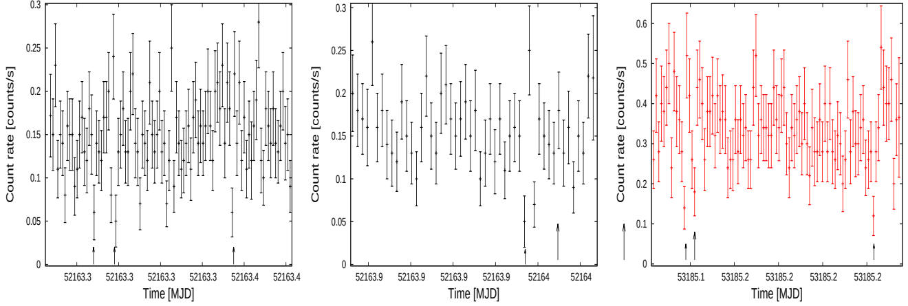
Figure 3. A zoom of the light curve, in the 0.3–10 keV energy band, sampled with a bin size of 100 seconds in the first (left, center) and 50 seconds in the second (right) Chandra observation. There may be marginal hints of dips at the times marked with black arrows.
