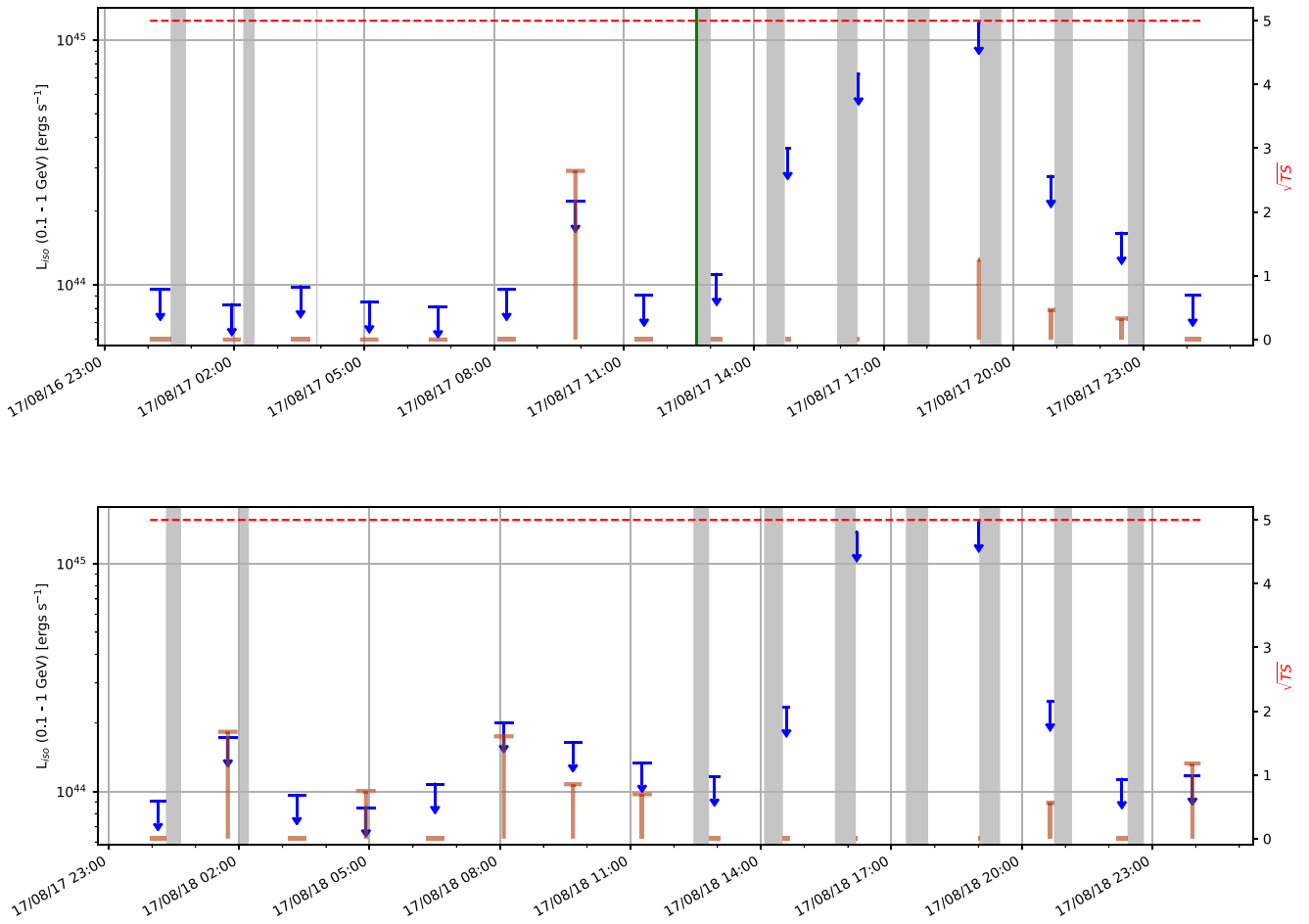
Figure 3. Luminosity in the 0.1–1 GeV energy range upper bounds (blue points, left y-axis) for the first 2 days after t_{\text{EM}} . The width of the blue points corresponds to the interval used in the analyses. The red bars of equivalent duration indicate the value of the significance (square root of the Test Statistic TS, right y-axis) in each interval, with the dashed red line representing a value corresponding to approximately 5\sigma ( \text{TS} = 25 ). The gray bands highlight the times when the LAT was in the SAA. The green vertical line in the upper panel is t_{\text{EM}} .
