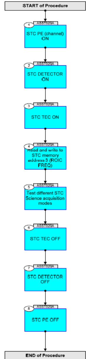
Figure 3 Procedure Flowchart Overview SS-TST-020
