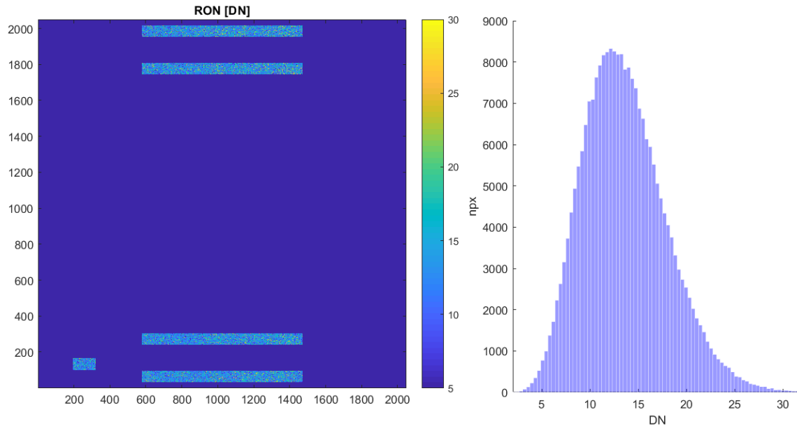
Figure 7 First image acquired during the functional tests: the windows acquired are the 4 broadband filters and the smaller mitigation window. Repetition time (RT)=400 ms, integration time (IT)=4 \mu s acquired. Left image shows the distribution (uniform) of the RON on the detector. On the right the distribution of the RON.
