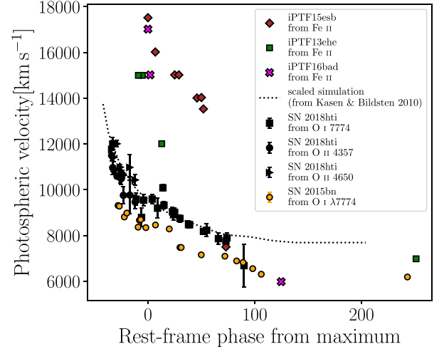
Figure 10. Photospheric velocities of SN 2018hti deduced from the absorption minima of O II \lambda 4357, 4650 (black dots and triangles) and O I \lambda 7774 (black squares) P-Cygni profiles (see the text). The evolution of the photospheric velocity of SN 2015bn (deduced by the O I, data taken from Nicholl et al. 2016, yellow dots), iPTF13ehe (green squares), iPTF15esb (brown diamonds), and iPTF16bad (magenta crosses) (deduced by the Fe II, Yan et al. 2017b) are shown for comparison. We also compared the photospheric velocity of SN 2018hti with the prediction of Kasen & Bildsten (2010) for a magnetar-powered SN (black dotted line, see the text).
