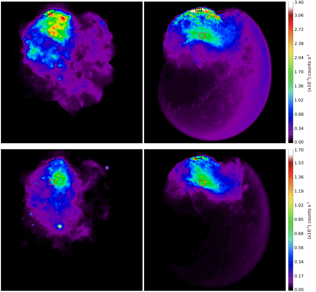
Fig. 9. Smoothed X-ray count rate maps in the [0.5–1.4] keV ( upper panels ) and [1.4–5] keV ( lower panels ) bands with a pixel size of 11". Left panels: 2010 observations resampled as explained in the Appendix B. Right panels: synthetic images derived from the model, as explained in Sect. 2.2. The black and red shapes indicate the regions selected for the spectra shown in Fig. 10.
