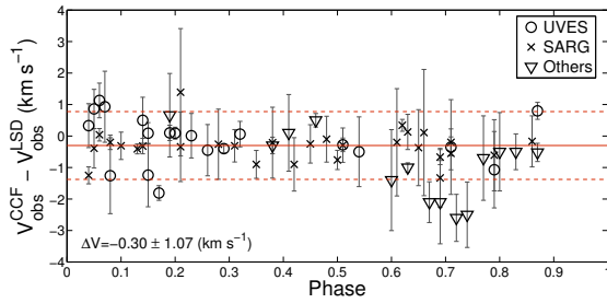
Figure 3. Differences between radial velocity estimates derived with the cross-correlation method, v_{obs}^{Cor} , and with the LSD profile method, v_{obs}^{LSD} . The observations from the different spectrographs are labeled respectively.
