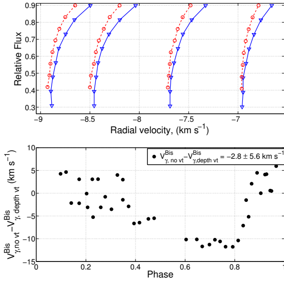
Figure 8. Top panel. Comparison of synthetic bisectors computed with the depth-dependent microturbulent velocity model (blue triangles) and with the constant microturbulent velocity v_{\text{mic}} = 2 \text{ km s}^{-1} (red circles). Bottom panel. The difference between the gamma velocities of RR Lyr derived with different sets of bisectors grid: with ( V_{\gamma}^{\text{Bis, depth-dep. } v_{\text{mic}}} ) and without depth-dependent v_{\text{mic}} stellar atmosphere models ( V_{\gamma, \text{RR Lyr}}^{\text{Bis, constant } v_{\text{mic}}} ).
