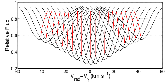
Figure 4. Example of LSD profiles and bisectors computed from model spectra of RR Lyrae (that corresponds to \phi=0.213 , or spectrum number 087 in Fossati et al. 2014) with pulsation velocities from -50 to +50 \text{ km s}^{-1} with a step 5 \text{ km s}^{-1} .
