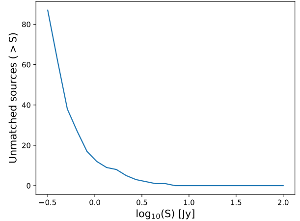
Fig. 5. Number of PCNT sources with no low-frequency counterpart as a function of the flux density at 30 GHz.
