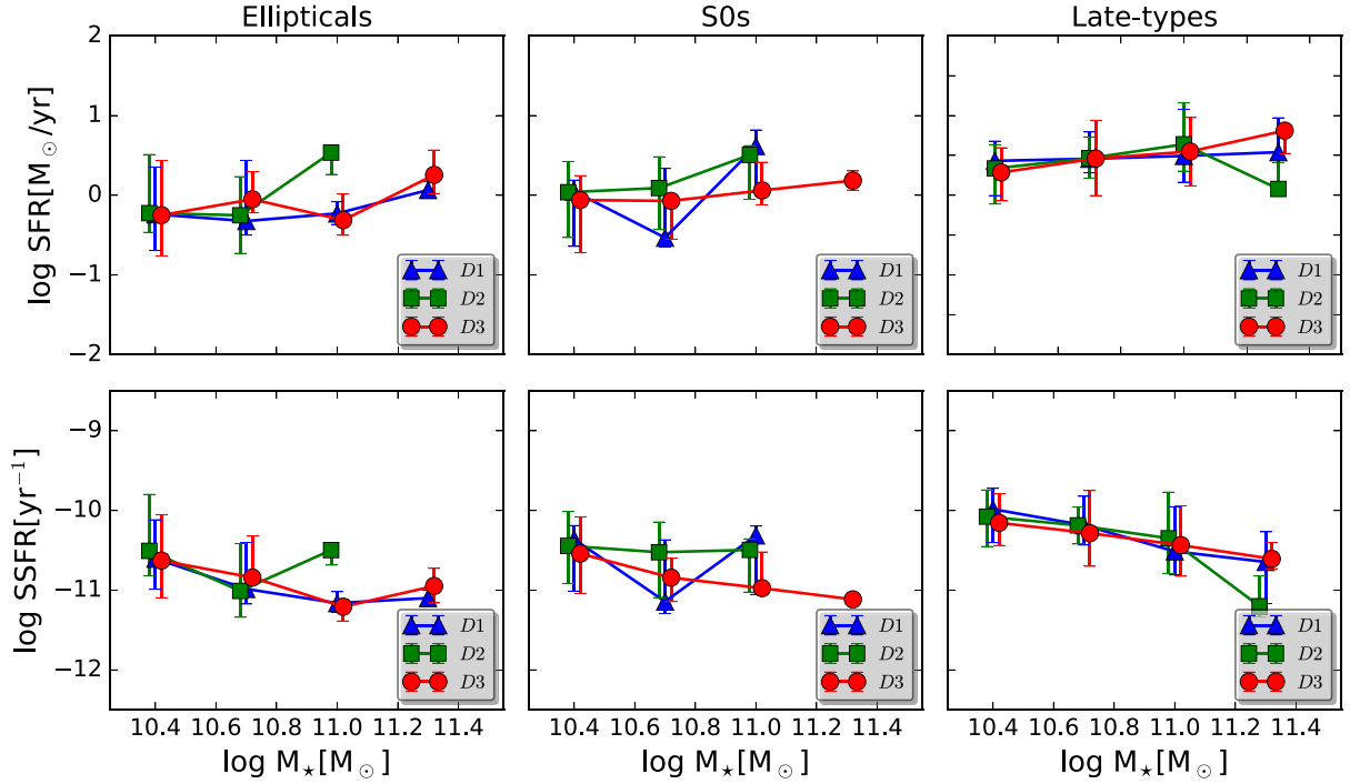
Figure 10. Comparison between the SFR- M_* and SSFR- M_* in the three bin of local density, D1 ( -2 \leq \text{LD} \leq -0.5 ), D2 ( -0.5 < \text{LD} < 0 ), and D3 ( 0 \leq \text{LD} \leq 1.8 ) fixing the morphological type. In each panel, the blue triangle points are the medians in the bin D1, the green squares points the medians in D2, and red circle points the ones in D3. Error bars represent the 25th and 75th percentiles.
