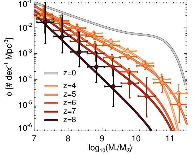
FIG. 13.— Redshift evolution of our fiducial GSMFs at z = 4-8 . For reference, the gray thick line denoting the z \sim 0 GSMF (Baldry et al. 2012) is shown.
