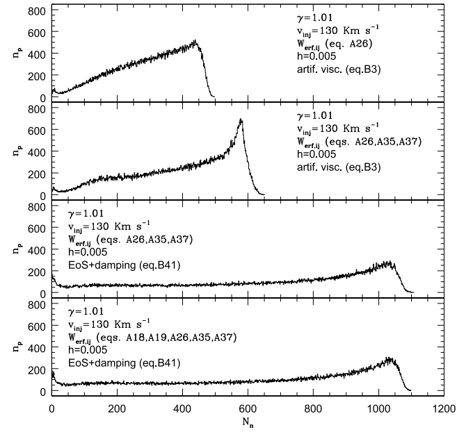
Fig. 17. Histograms showing, for the four SPH W_{\text{erf},ij} models of Fig. 16, the distribution of particles n_p relative to their companions N_n within the radial interpolation extension 4h .
