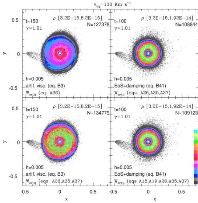
Fig. 16. xy scatter plots in a linear scale of 16 colours of 3D SPH non-viscous accretion disc models for W_{\text{erf},ij} . Colours refer to the dimensionless mass-density \rho . Data identifying the SPH modelling are also reported with references to the Appendices, together with the dimensionless lower and upper \rho values of the colour bar, within the square brackets: [\rho_{\min}, \rho_{\max}] at the top of each panel. Dots in dark grey (bottom of the colour bar) refer to values of \rho \leq \rho_{\min} . Dots in cyan (top of the colour bar) refer to values of \rho \geq \rho_{\max} . As for \rho_{\min} and \rho_{\max} , the computer exponential notation is used instead of the scientific exponential notation. All N particles are also reported in each panel. v_{\text{inj}} is reported on top of the entire figure. Numerical values alongside the colour bar are not reported for practical reasons. The \rho values within to the n th colour of the colour bar are computed as \rho_n = \rho_{\min} + (n-2)(\rho_{\max} - \rho_{\min})/14 and \rho_{n+1} = \rho_{\min} + (n-1)(\rho_{\max} - \rho_{\min})/14 , n = 2, 3, \dots, 15 .
