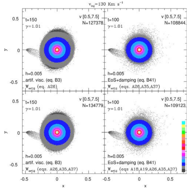
Fig. 19. xy scatter plots in a linear scale of 16 colours of 3D SPH non-viscous accretion disc models of Fig. 16. Colours refer to the dimensionless total velocity v . Data identifying the SPH modelling are also reported with references to the Appendices, together with the dimensionless lower and upper v values of the colour bar, within the square brackets: [v_{min}, v_{max}] on top of each panel. Dots in dark grey (bottom of the colour bar) refer to values of v \leq v_{min} . Dots in cyan (top of the colour bar) refer to values of v \geq v_{max} . All N particles are also reported in each panel. v_{inj} is reported on top of the entire figure. Numerical values alongside the colour bar are not reported for practical reasons. The v values within to the n th colour of the colour bar are computed as v_n = v_{min} + (n-2)(v_{max} - v_{min})/14 and v_{n+1} = v_{min} + (n-1)(v_{max} - v_{min})/14 , n = 2, 3, \dots, 15 .
