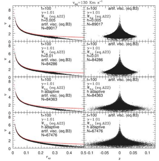
Fig. 25. r_{xy} radial and z vertical distributions of dimensionless values of v for accretion disc models of Fig. 13. In each panel some modelling data are reported, together with references (in the Appendices) regarding both the numerical normalization and the dissipation. v_{inj} is reported on top of the entire figure. In the left-side panels, regarding the radial distribution, some profiles in red are also shown for comparison, each relative to the Keplerian kinematics profile.
