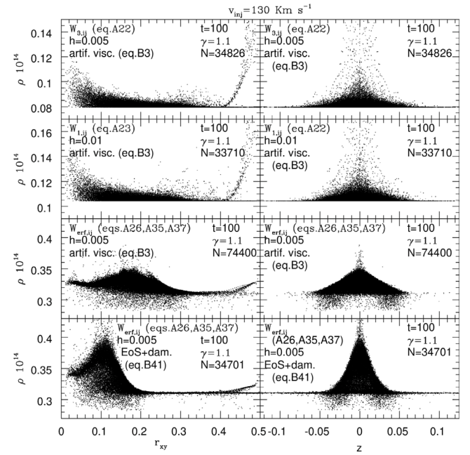
Fig. 8. r_{xy} radial and z vertical distributions of dimensionless values of (\rho 10^{-14}) for the most significant accretion disc models of Figs. 1 and 3. In each panel some modelling data are reported, together with references (in the Appendices) regarding both the numerical normalization and the dissipation. v_{\text{inj}} is reported on top of the entire figure.
