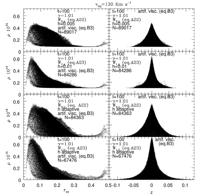
Fig. 21. r_{xy} radial and z vertical distributions of dimensionless values of \rho 10^{14} for accretion disc models of Fig. 11. In each panel some modelling data are reported, together with references (in the Appendices) regarding the dissipation. v_{inj} is reported on top of the entire figure.
