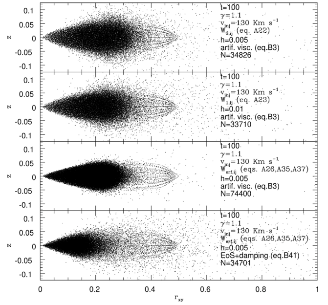
Fig. 5. (r_{xy}, z) plots for the most significant models of Figs. 1 and 3. All disc modelling data are reported for each panel.
