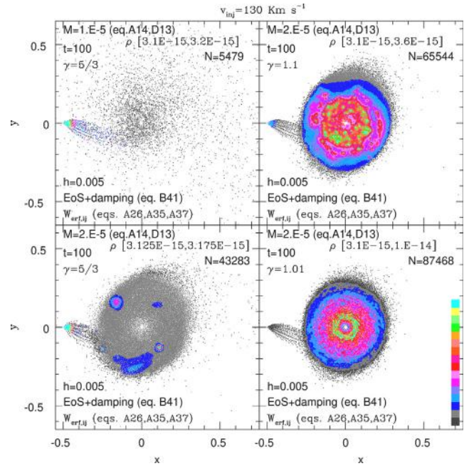
Fig. 27. xy scatter plots in a linear scale of 16 colours of 3D SPH viscous accretion disc models for W_{\text{erf},ij} . Colours refer to the dimensionless mass-density \rho . Data identifying the SPH modelling are also reported with references to the Appendices, together with the dimensionless lower and upper \rho values of the colour bar: [\rho_{\min}, \rho_{\max}] at the top of each panel. Dots in dark grey (bottom of the colour bar) refer to values of \rho \leq \rho_{\min} . Dots in cyan (top of the colour bar) refer to values of \rho \geq \rho_{\max} . As for \rho_{\min} and \rho_{\max} , the computer exponential notation is used instead of the scientific exponential notation. All N particles are also reported in each panel. v_{\text{inj}} is reported on top of the entire figure. Numerical values alongside the colour bar are not reported for practical reasons. The \rho values within to the n th colour of the colour bar are computed as \rho_n = \rho_{\min} + (n-2)(\rho_{\max} - \rho_{\min})/14 and \rho_{n+1} = \rho_{\min} + (n-1)(\rho_{\max} - \rho_{\min})/14 , n = 2, 3, \dots, 15 .
